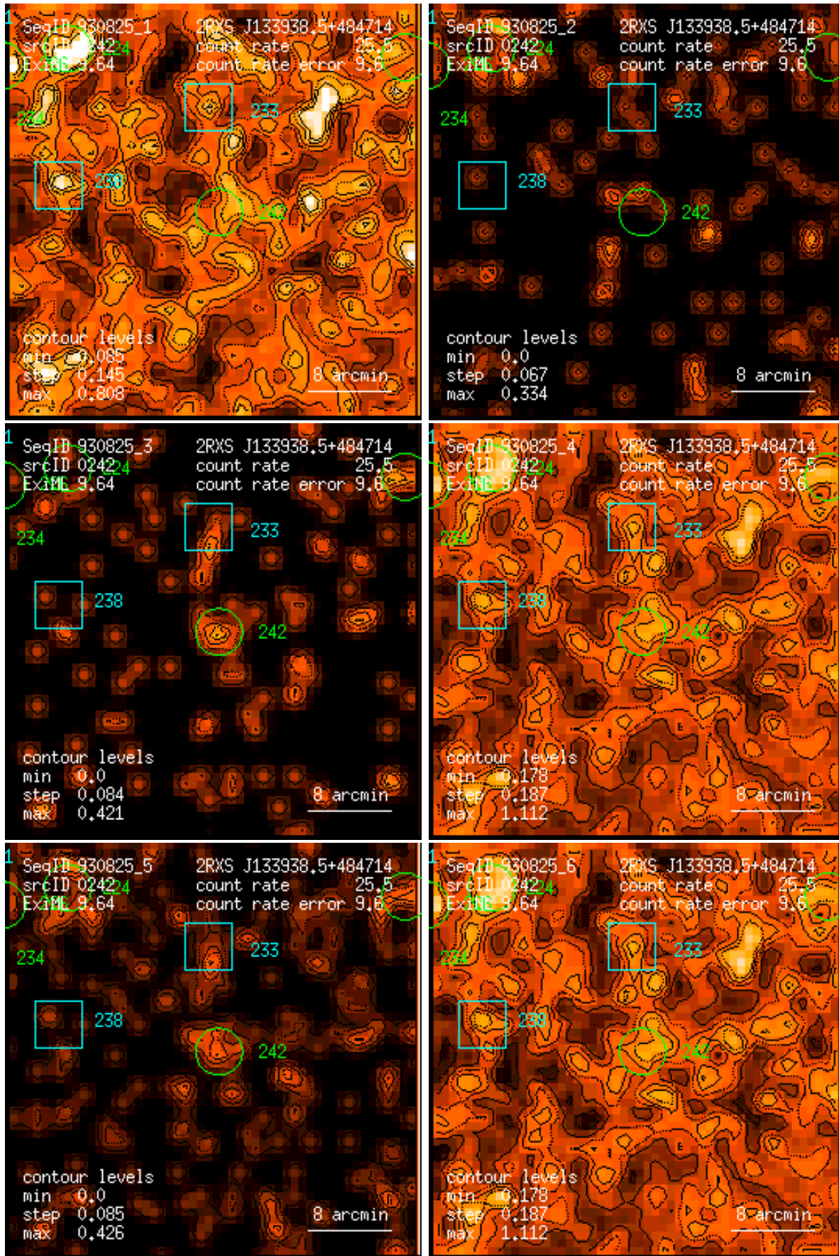
Figure 242: RASS 930825: detection 0242: band rate images, Gaussian filter: (1) PSPC channels 11 – 41, (2) 52 – 90, (3) 91 – 201, (4) 11 – 235, (5) 52 – 201, (6) 11 – 201. Broad band rates in counts/ks. Band rate contour levels in counts/ks/arcmin 2 .
