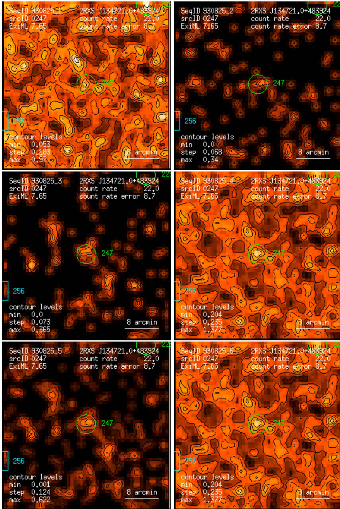
Figure 247: RASS 930825: detection 0247: band rate images, Gaussian filter: (1) PSPC channels 11 – 41, (2) 52 – 90, (3) 91 – 201, (4) 11 – 235, (5) 52 – 201, (6) 11 – 201. Broad band rates in counts/ks. Band rate contour levels in counts/ks/arcmin 2 .
