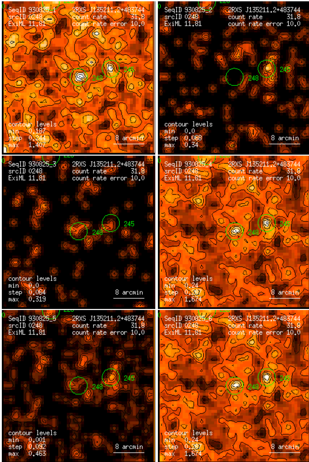
Figure 248: RASS 930825: detection 0248: band rate images, Gaussian filter: (1) PSPC channels 11 – 41, (2) 52 – 90, (3) 91 – 201, (4) 11 – 235, (5) 52 – 201, (6) 11 – 201. Broad band rates in counts/ks. Band rate contour levels in counts/ks/arcmin 2 .
