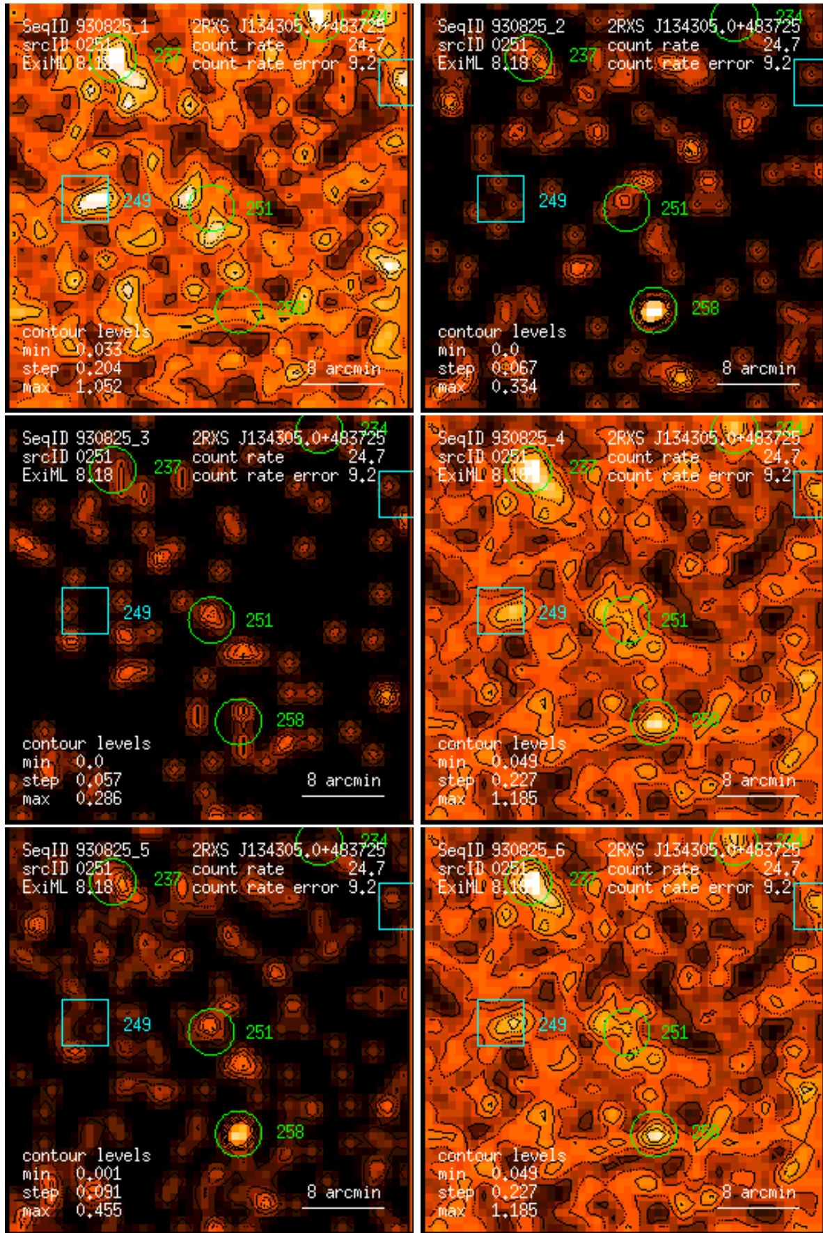
Figure 251: RASS 930825: detection 0251: band rate images, Gaussian filter: (1) PSPC channels 11 – 41, (2) 52 – 90, (3) 91 – 201, (4) 11 – 235, (5) 52 – 201, (6) 11 – 201. Broad band rates in counts/ks. Band rate contour levels in counts/ks/arcmin 2 .
