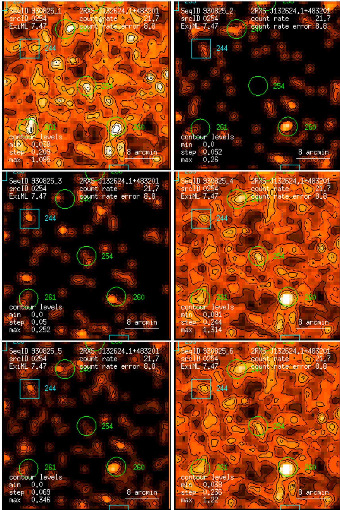
Figure 254: RASS 930825: detection 0254: band rate images, Gaussian filter: (1) PSPC channels 11 – 41, (2) 52 – 90, (3) 91 – 201, (4) 11 – 235, (5) 52 – 201, (6) 11 – 201. Broad band rates in counts/ks. Band rate contour levels in counts/ks/arcmin 2 .
