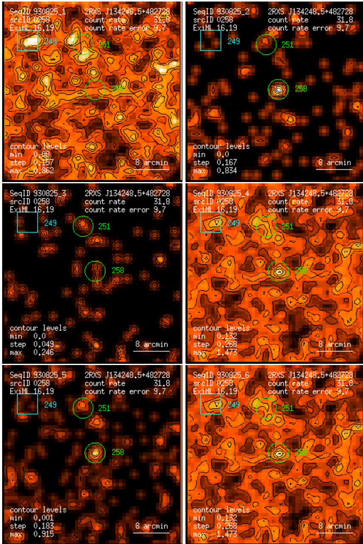
Figure 258: RASS 930825: detection 0258: band rate images, Gaussian filter: (1) PSPC channels 11 – 41, (2) 52 – 90, (3) 91 – 201, (4) 11 – 235, (5) 52 – 201, (6) 11 – 201. Broad band rates in counts/ks. Band rate contour levels in counts/ks/arcmin 2 .
