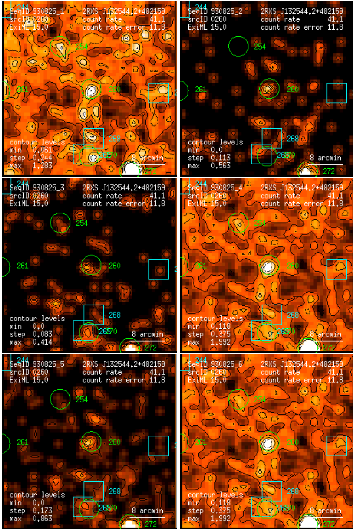
Figure 260: RASS 930825: detection 0260: band rate images, Gaussian filter: (1) PSPC channels 11 – 41, (2) 52 – 90, (3) 91 – 201, (4) 11 – 235, (5) 52 – 201, (6) 11 – 201. Broad band rates in counts/ks. Band rate contour levels in counts/ks/arcmin 2 .
