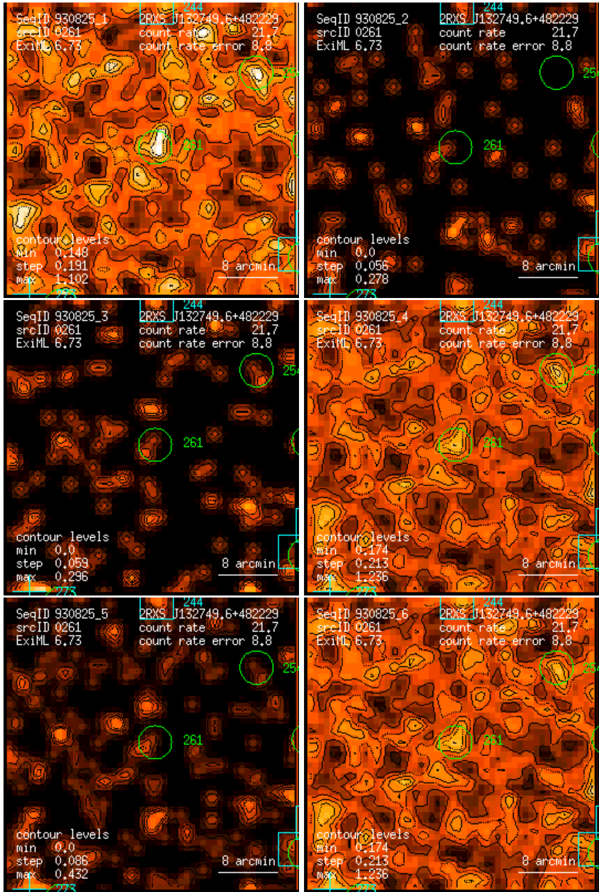
Figure 261: RASS 930825: detection 0261: band rate images, Gaussian filter: (1) PSPC channels 11 – 41, (2) 52 – 90, (3) 91 – 201, (4) 11 – 235, (5) 52 – 201, (6) 11 – 201. Broad band rates in counts/ks. Band rate contour levels in counts/ks/arcmin 2 .
