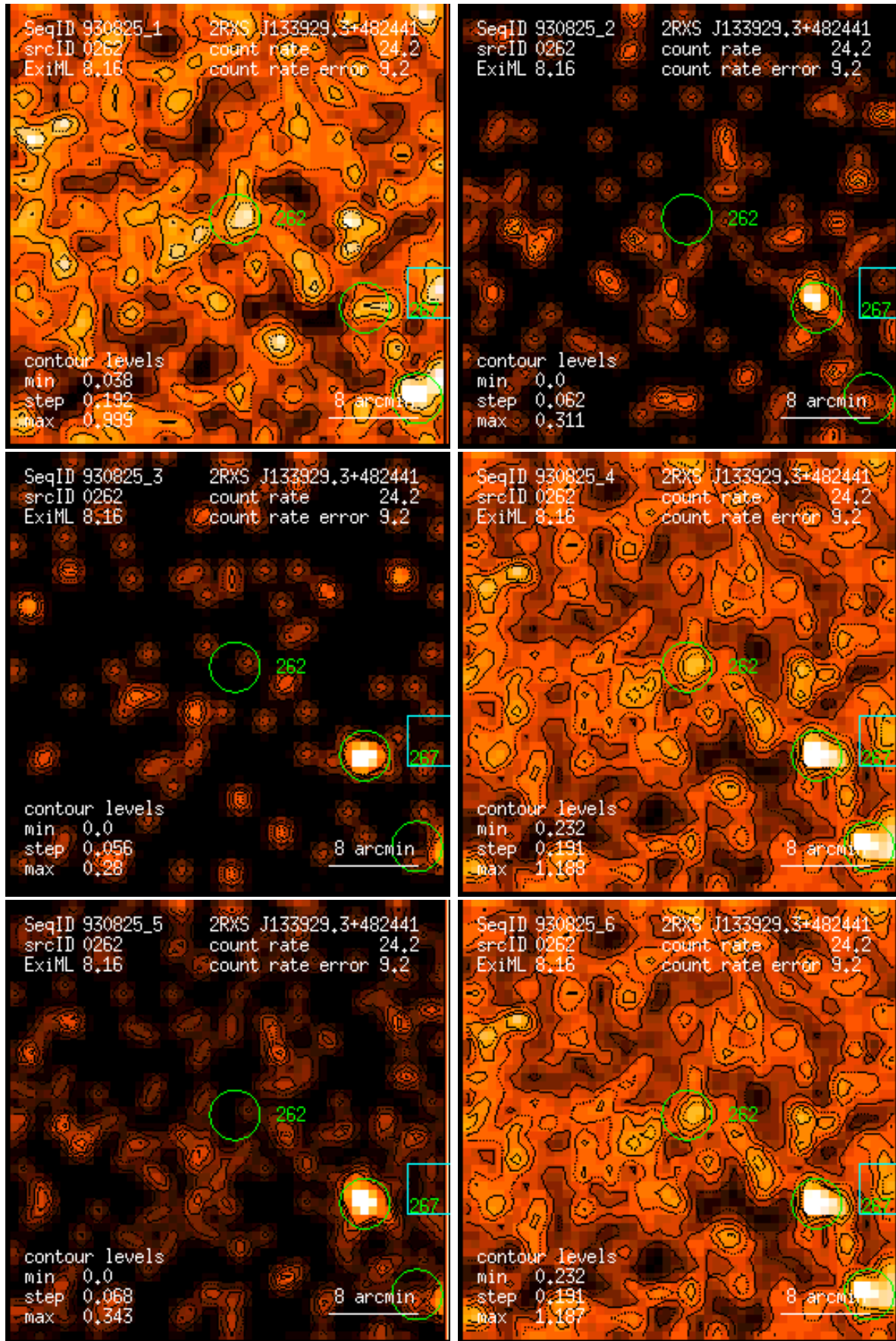
Figure 262: RASS 930825: detection 0262: band rate images, Gaussian filter: (1) PSPC channels 11 – 41, (2) 52 – 90, (3) 91 – 201, (4) 11 – 235, (5) 52 – 201, (6) 11 – 201. Broad band rates in counts/ks. Band rate contour levels in counts/ks/arcmin 2 .
