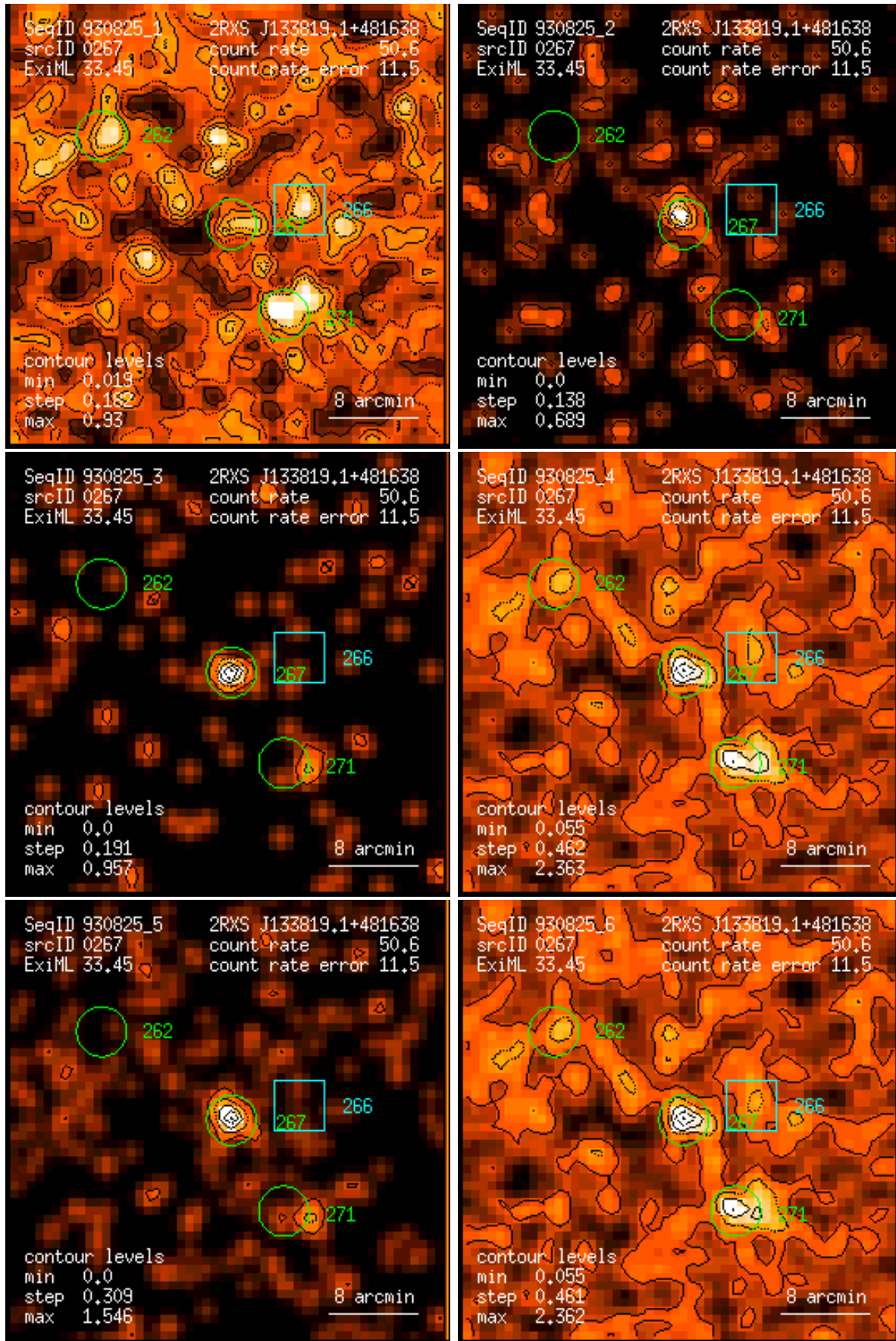
Figure 267: RASS 930825: detection 0267: band rate images, Gaussian filter: (1) PSPC channels 11 – 41, (2) 52 – 90, (3) 91 – 201, (4) 11 – 235, (5) 52 – 201, (6) 11 – 201. Broad band rates in counts/ks. Band rate contour levels in counts/ks/arcmin 2 .
