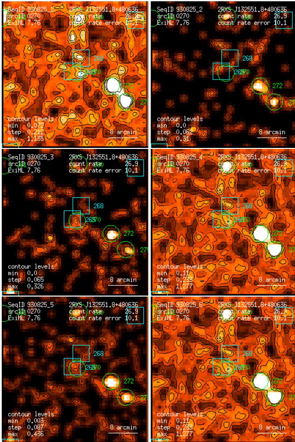
Figure 270: RASS 930825: detection 0270: band rate images, Gaussian filter: (1) PSPC channels 11 – 41, (2) 52 – 90, (3) 91 – 201, (4) 11 – 235, (5) 52 – 201, (6) 11 – 201. Broad band rates in counts/ks. Band rate contour levels in counts/ks/arcmin 2 .
