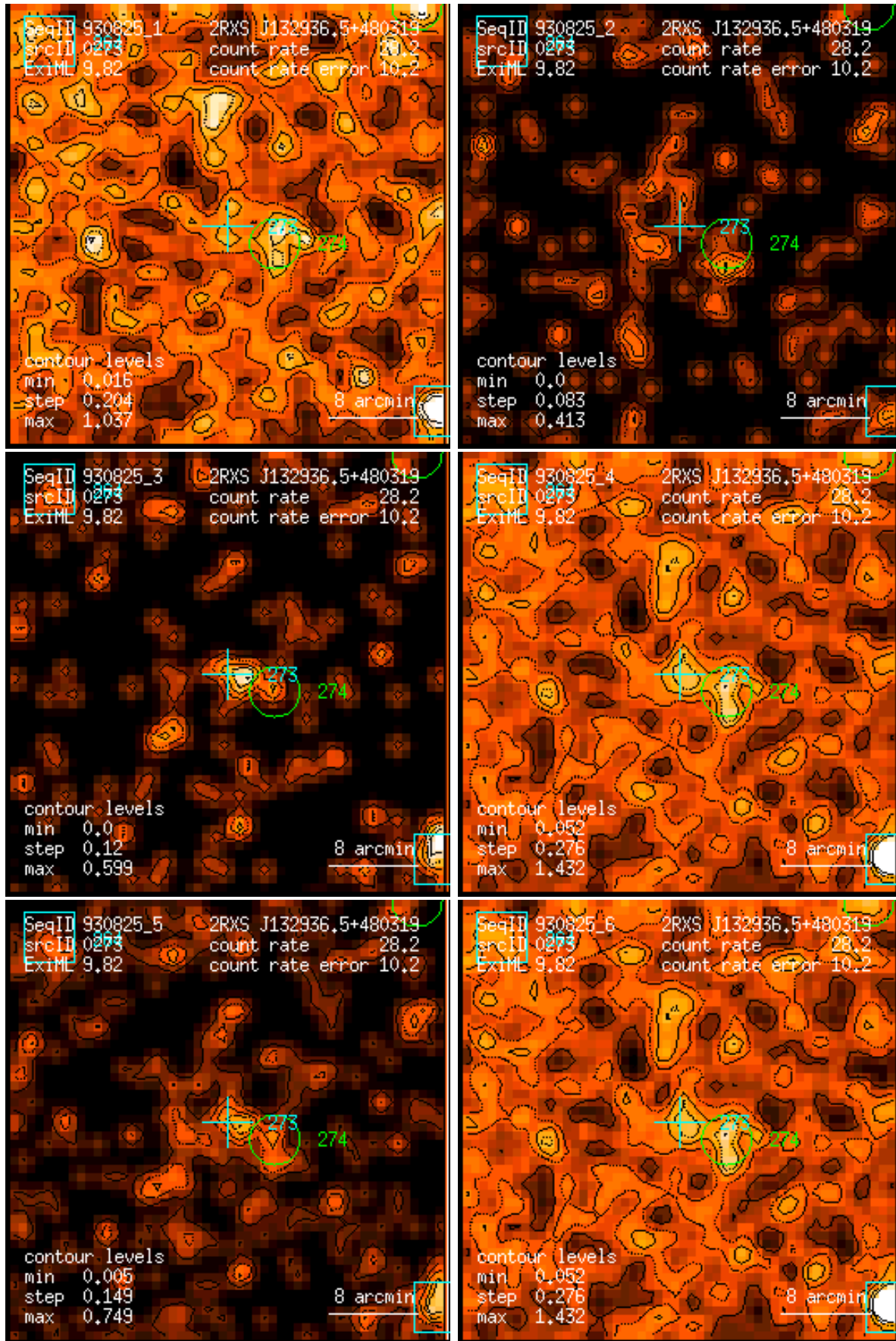
Figure 273: RASS 930825: detection 0273: band rate images, Gaussian filter: (1) PSPC channels 11 – 41, (2) 52 – 90, (3) 91 – 201, (4) 11 – 235, (5) 52 – 201, (6) 11 – 201. Broad band rates in counts/ks. Band rate contour levels in counts/ks/arcmin 2 .
