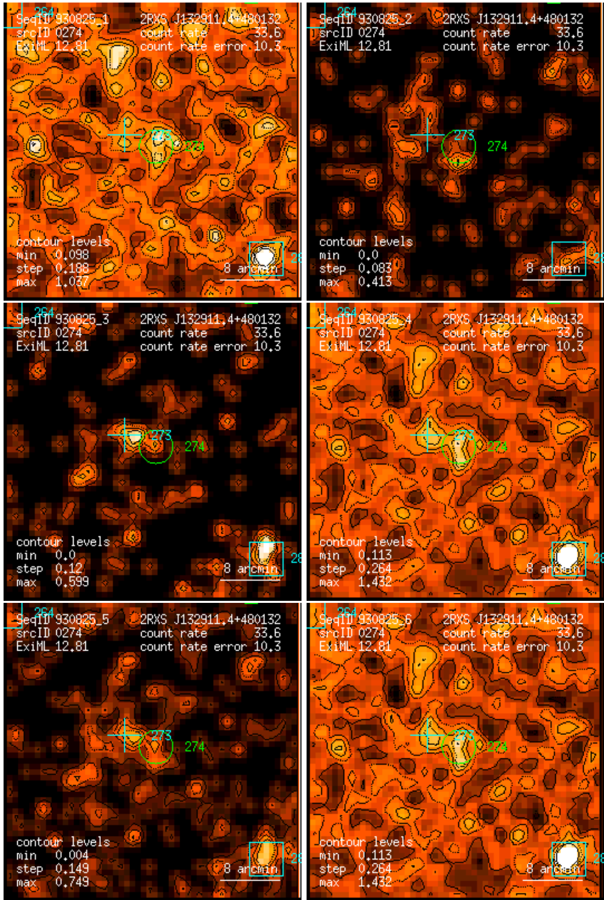
Figure 274: RASS 930825: detection 0274: band rate images, Gaussian filter: (1) PSPC channels 11 – 41, (2) 52 – 90, (3) 91 – 201, (4) 11 – 235, (5) 52 – 201, (6) 11 – 201. Broad band rates in counts/ks. Band rate contour levels in counts/ks/arcmin 2 .
