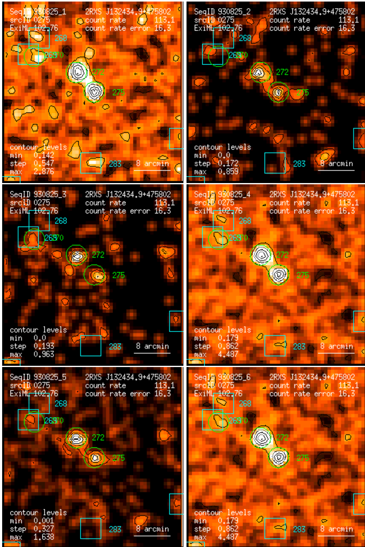
Figure 275: RASS 930825: detection 0275: band rate images, Gaussian filter: (1) PSPC channels 11 – 41, (2) 52 – 90, (3) 91 – 201, (4) 11 – 235, (5) 52 – 201, (6) 11 – 201. Broad band rates in counts/ks. Band rate contour levels in counts/ks/arcmin 2 .
