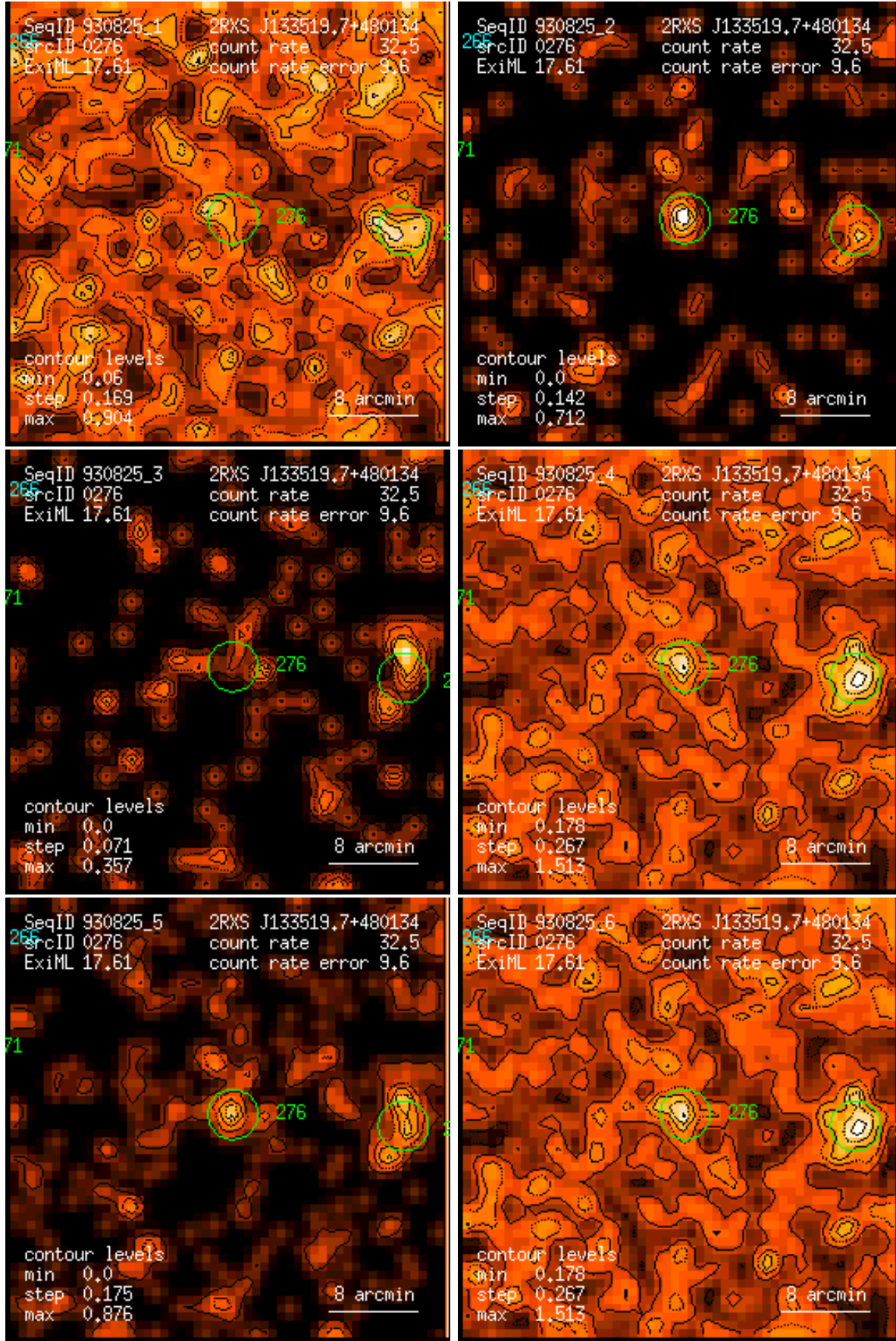
Figure 276: RASS 930825: detection 0276: band rate images, Gaussian filter: (1) PSPC channels 11 – 41, (2) 52 – 90, (3) 91 – 201, (4) 11 – 235, (5) 52 – 201, (6) 11 – 201. Broad band rates in counts/ks. Band rate contour levels in counts/ks/arcmin 2 .
