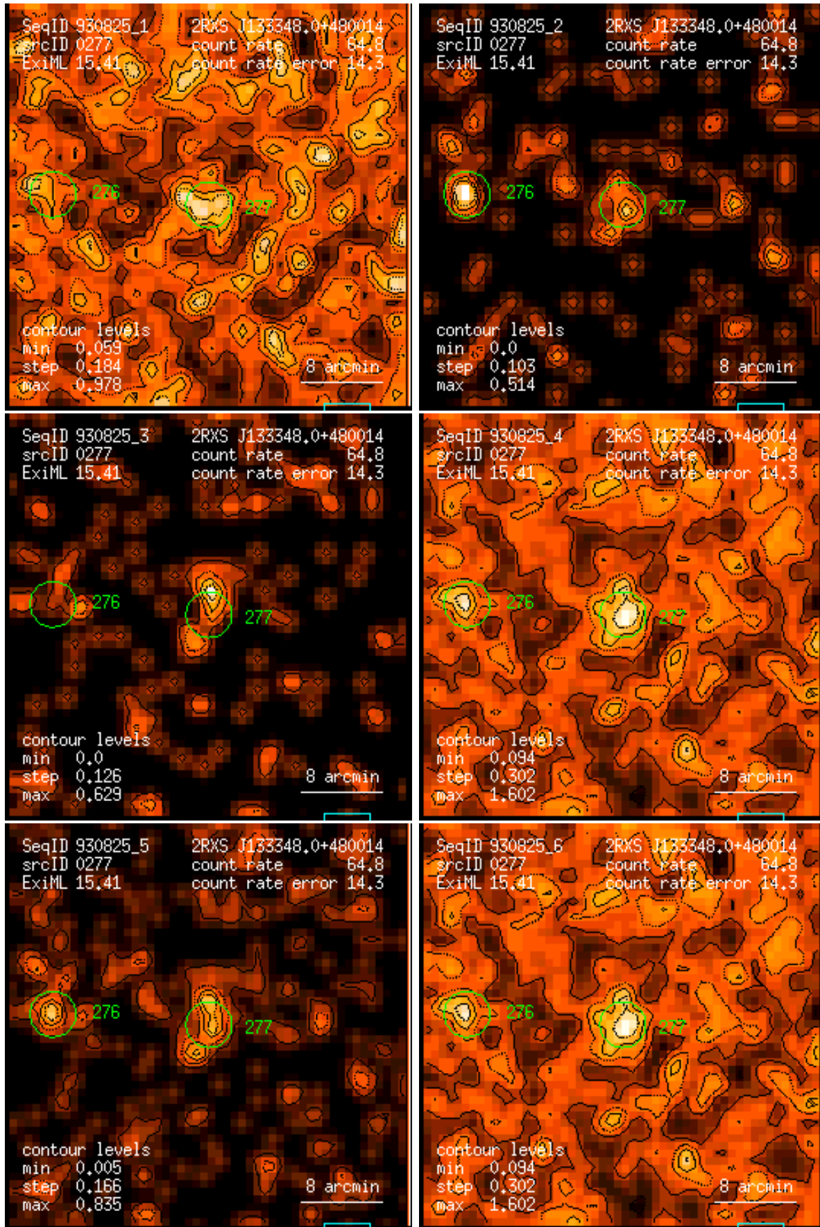
Figure 277: RASS 930825: detection 0277: band rate images, Gaussian filter: (1) PSPC channels 11 – 41, (2) 52 – 90, (3) 91 – 201, (4) 11 – 235, (5) 52 – 201, (6) 11 – 201. Broad band rates in counts/ks. Band rate contour levels in counts/ks/arcmin 2 .
