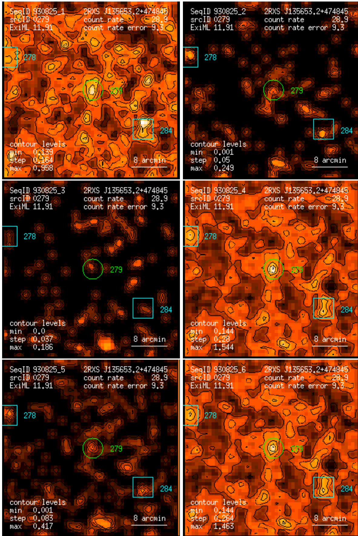
Figure 279: RASS 930825: detection 0279: band rate images, Gaussian filter: (1) PSPC channels 11 – 41, (2) 52 – 90, (3) 91 – 201, (4) 11 – 235, (5) 52 – 201, (6) 11 – 201. Broad band rates in counts/ks. Band rate contour levels in counts/ks/arcmin 2 .
