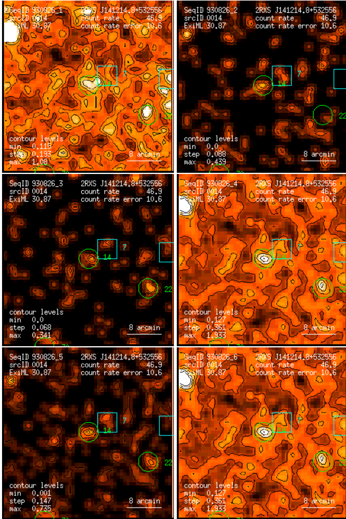
Figure 14: RASS 930826: detection 0014: band rate images, Gaussian filter: (1) PSPC channels 11 – 41, (2) 52 – 90, (3) 91 – 201, (4) 11 – 235, (5) 52 – 201, (6) 11 – 201. Broad band rates in counts/ks. Band rate contour levels in counts/ks/arcmin 2 .
