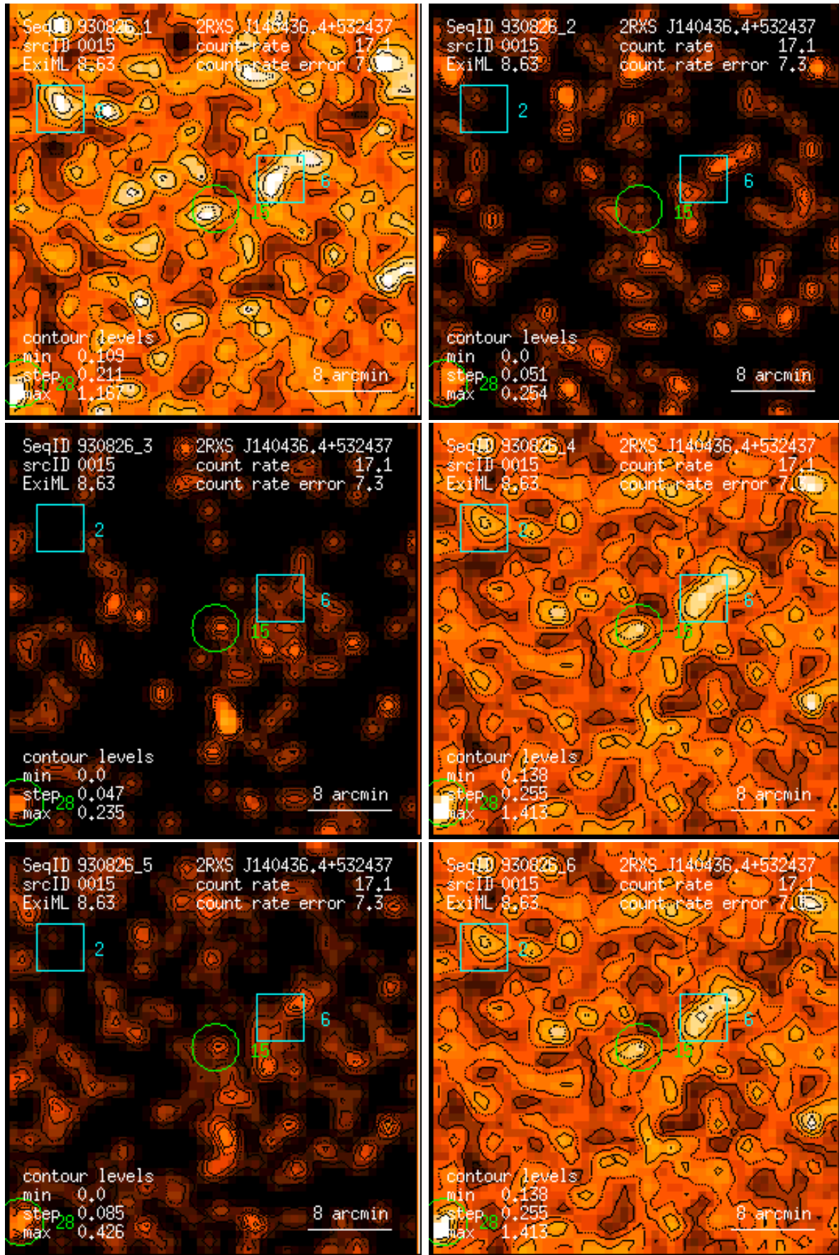
Figure 15: RASS 930826: detection 0015: band rate images, Gaussian filter: (1) PSPC channels 11 – 41, (2) 52 – 90, (3) 91 – 201, (4) 11 – 235, (5) 52 – 201, (6) 11 – 201. Broad band rates in counts/ks. Band rate contour levels in counts/ks/arcmin 2 .
