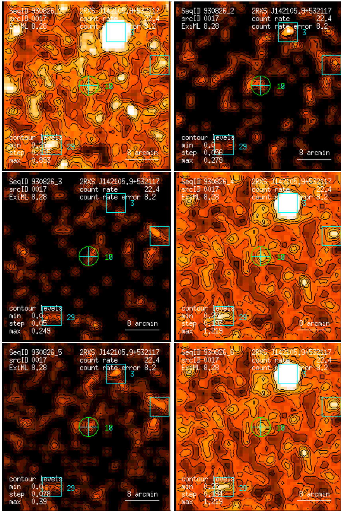
Figure 17: RASS 930826: detection 0017: band rate images, Gaussian filter: (1) PSPC channels 11 – 41, (2) 52 – 90, (3) 91 – 201, (4) 11 – 235, (5) 52 – 201, (6) 11 – 201. Broad band rates in counts/ks. Band rate contour levels in counts/ks/arcmin 2 .
