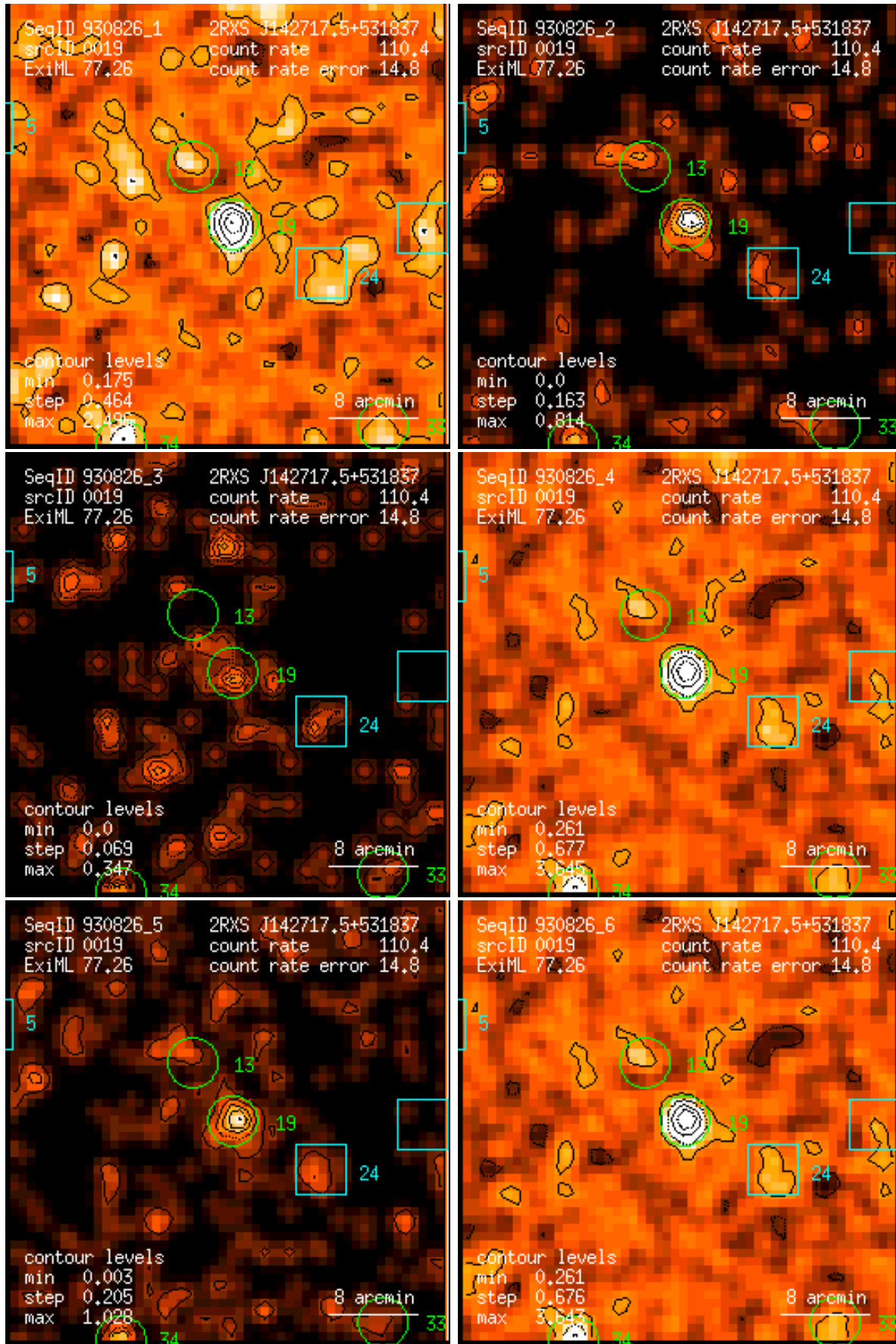
Figure 19: RASS 930826: detection 0019: band rate images, Gaussian filter: (1) PSPC channels 11 – 41, (2) 52 – 90, (3) 91 – 201, (4) 11 – 235, (5) 52 – 201, (6) 11 – 201. Broad band rates in counts/ks. Band rate contour levels in counts/ks/arcmin 2 .
