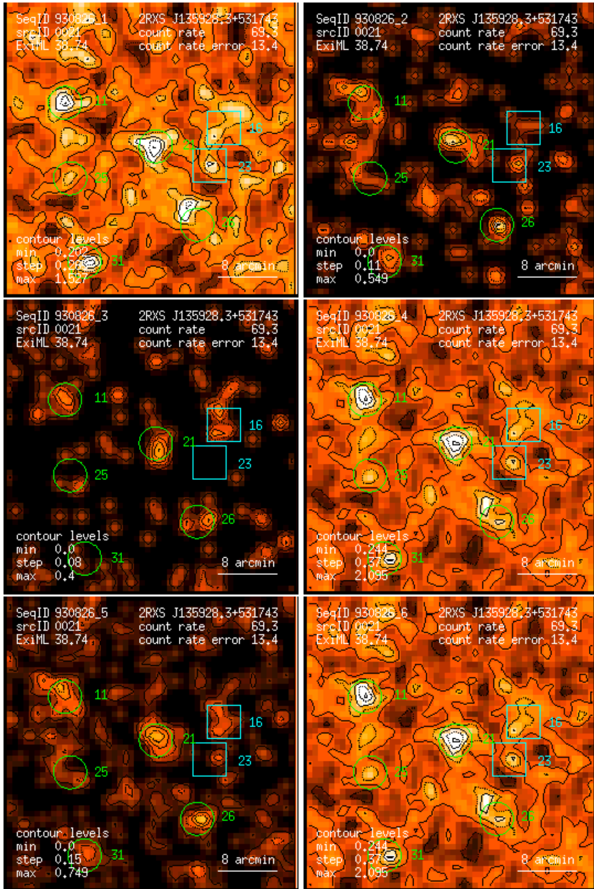
Figure 21: RASS 930826: detection 0021: band rate images, Gaussian filter: (1) PSPC channels 11 – 41, (2) 52 – 90, (3) 91 – 201, (4) 11 – 235, (5) 52 – 201, (6) 11 – 201. Broad band rates in counts/ks. Band rate contour levels in counts/ks/arcmin 2 .
