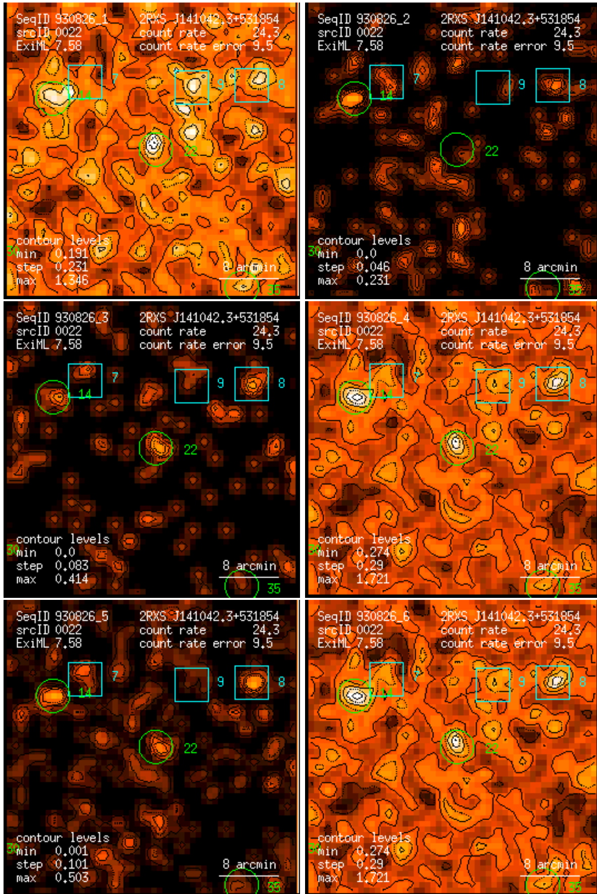
Figure 22: RASS 930826: detection 0022: band rate images, Gaussian filter: (1) PSPC channels 11 – 41, (2) 52 – 90, (3) 91 – 201, (4) 11 – 235, (5) 52 – 201, (6) 11 – 201. Broad band rates in counts/ks. Band rate contour levels in counts/ks/arcmin 2 .
