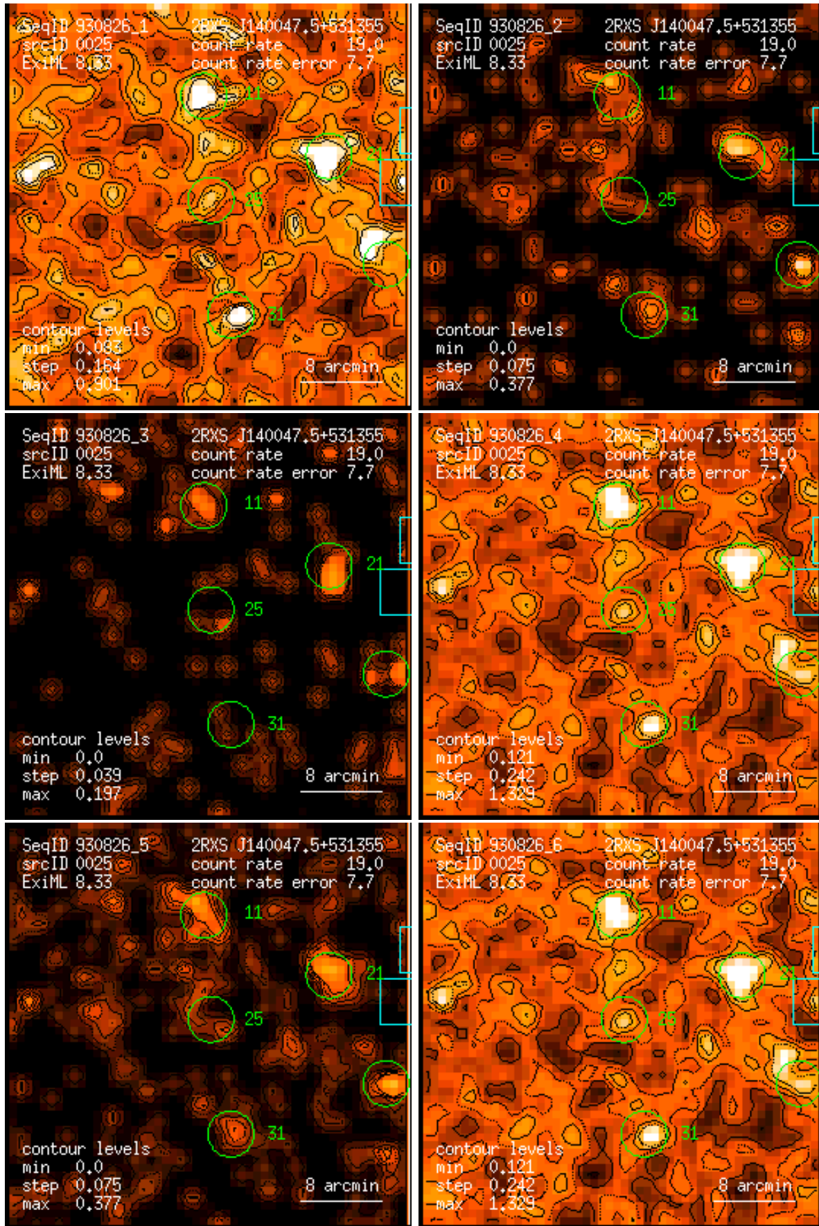
Figure 25: RASS 930826: detection 0025: band rate images, Gaussian filter: (1) PSPC channels 11 – 41, (2) 52 – 90, (3) 91 – 201, (4) 11 – 235, (5) 52 – 201, (6) 11 – 201. Broad band rates in counts/ks. Band rate contour levels in counts/ks/arcmin 2 .
