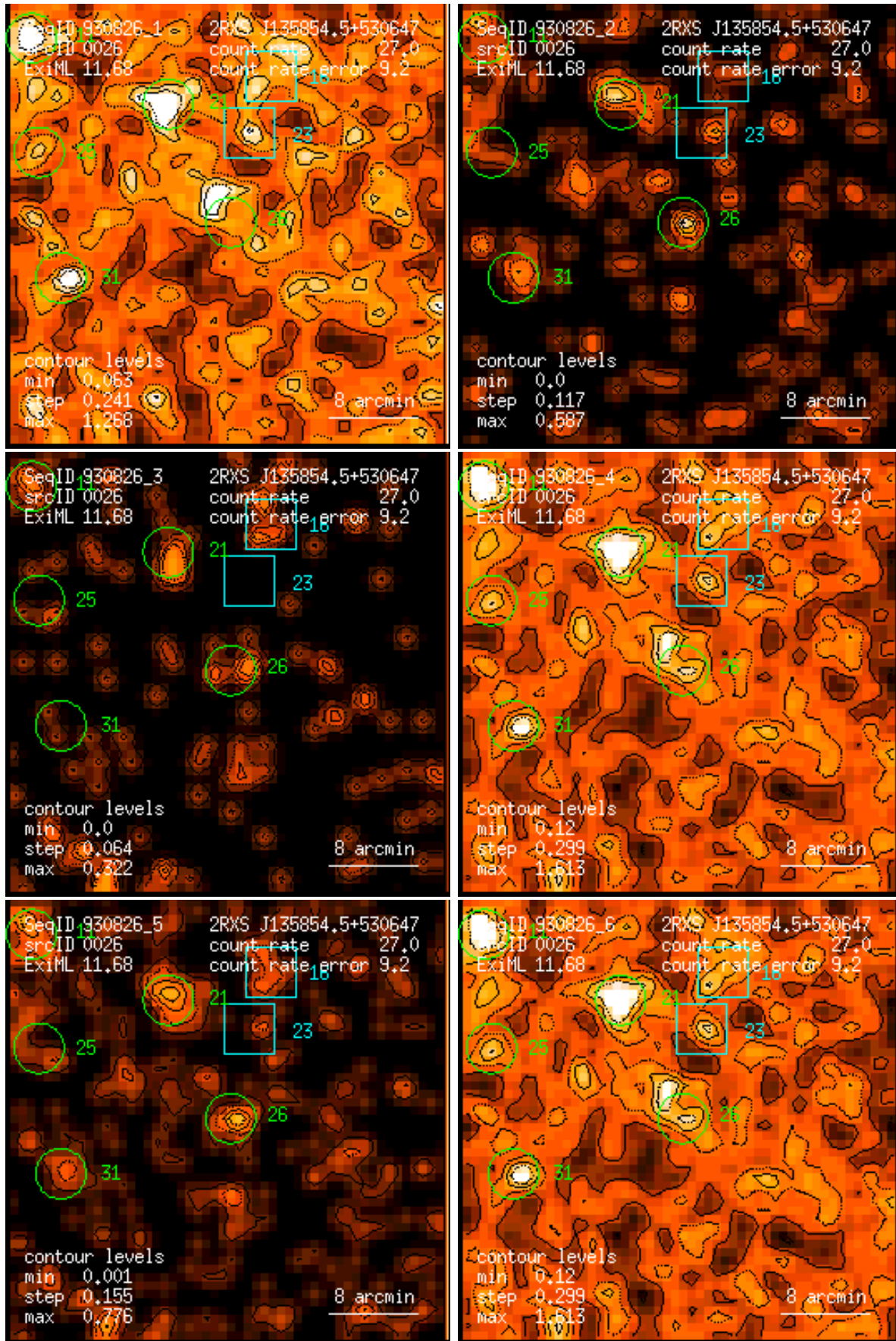
Figure 26: RASS 930826: detection 0026: band rate images, Gaussian filter: (1) PSPC channels 11 – 41, (2) 52 – 90, (3) 91 – 201, (4) 11 – 235, (5) 52 – 201, (6) 11 – 201. Broad band rates in counts/ks. Band rate contour levels in counts/ks/arcmin 2 .
