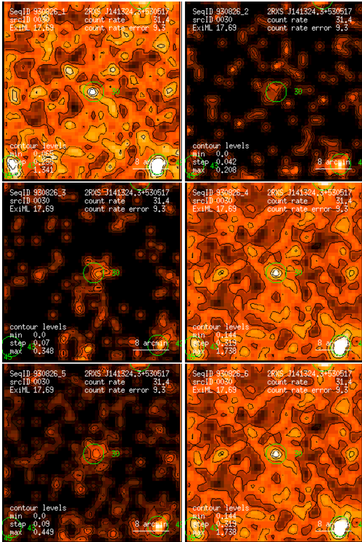
Figure 30: RASS 930826: detection 0030: band rate images, Gaussian filter: (1) PSPC channels 11 – 41, (2) 52 – 90, (3) 91 – 201, (4) 11 – 235, (5) 52 – 201, (6) 11 – 201. Broad band rates in counts/ks. Band rate contour levels in counts/ks/arcmin 2 .
