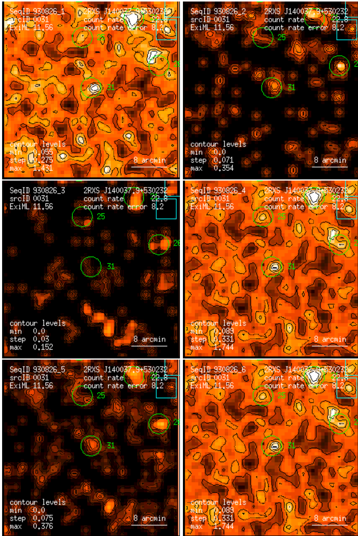
Figure 31: RASS 930826: detection 0031: band rate images, Gaussian filter: (1) PSPC channels 11 – 41, (2) 52 – 90, (3) 91 – 201, (4) 11 – 235, (5) 52 – 201, (6) 11 – 201. Broad band rates in counts/ks. Band rate contour levels in counts/ks/arcmin 2 .
