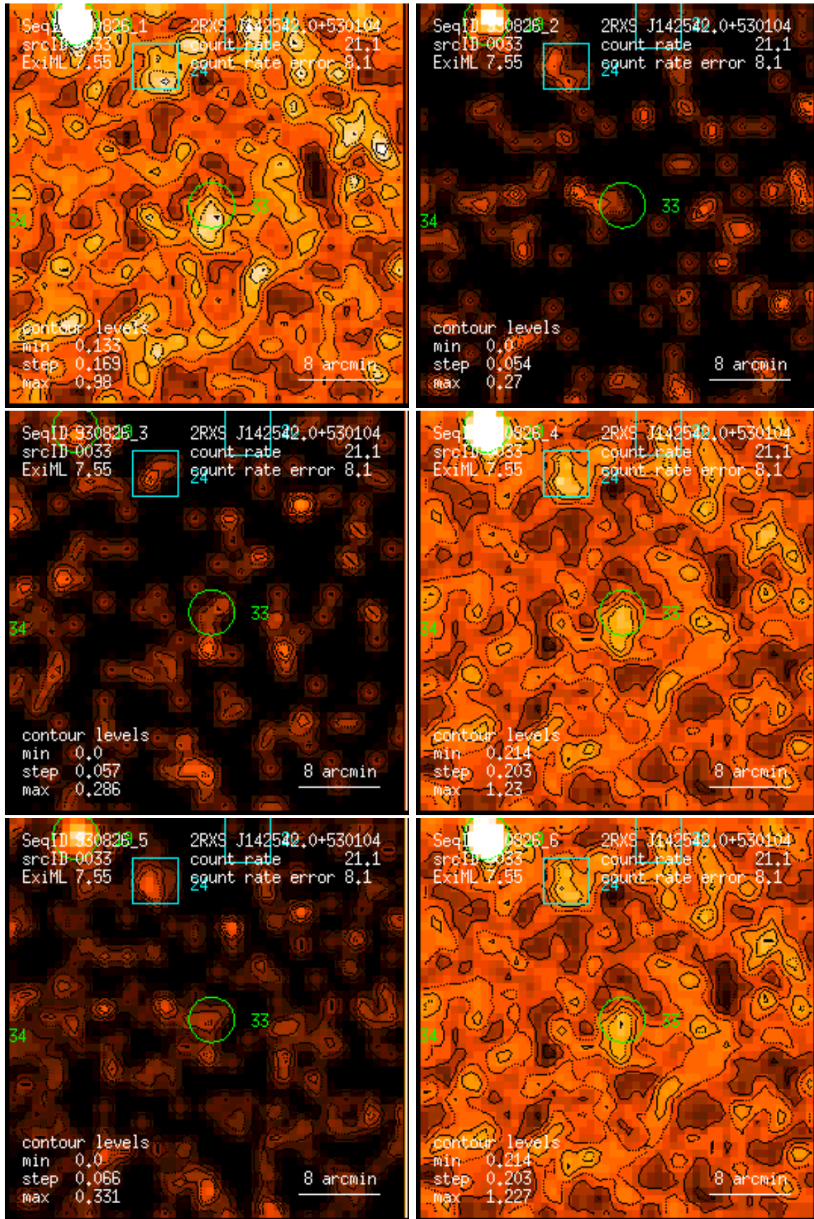
Figure 33: RASS 930826: detection 0033: band rate images, Gaussian filter: (1) PSPC channels 11 – 41, (2) 52 – 90, (3) 91 – 201, (4) 11 – 235, (5) 52 – 201, (6) 11 – 201. Broad band rates in counts/ks. Band rate contour levels in counts/ks/arcmin 2 .
