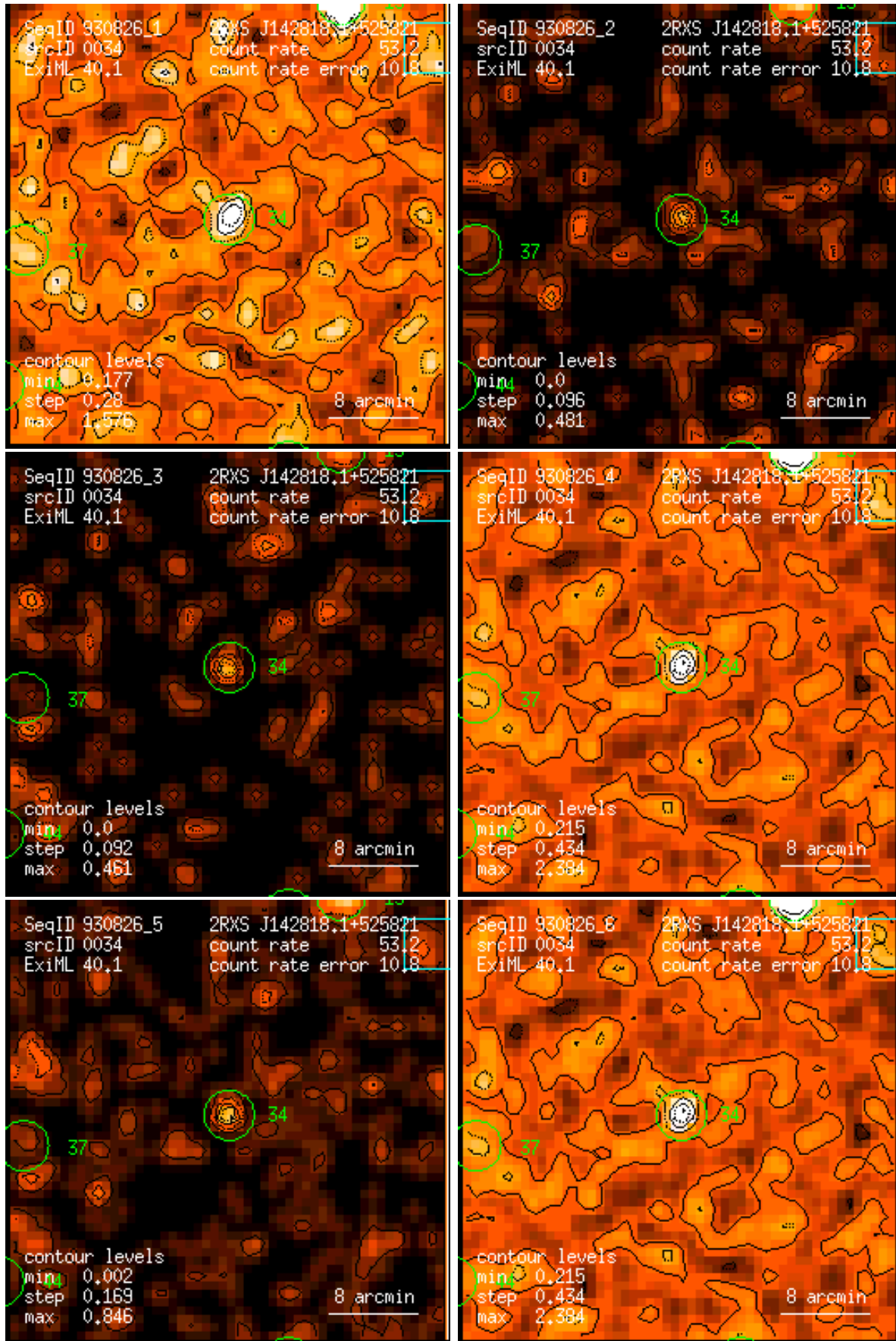
Figure 34: RASS 930826: detection 0034: band rate images, Gaussian filter: (1) PSPC channels 11 – 41, (2) 52 – 90, (3) 91 – 201, (4) 11 – 235, (5) 52 – 201, (6) 11 – 201. Broad band rates in counts/ks. Band rate contour levels in counts/ks/arcmin 2 .
