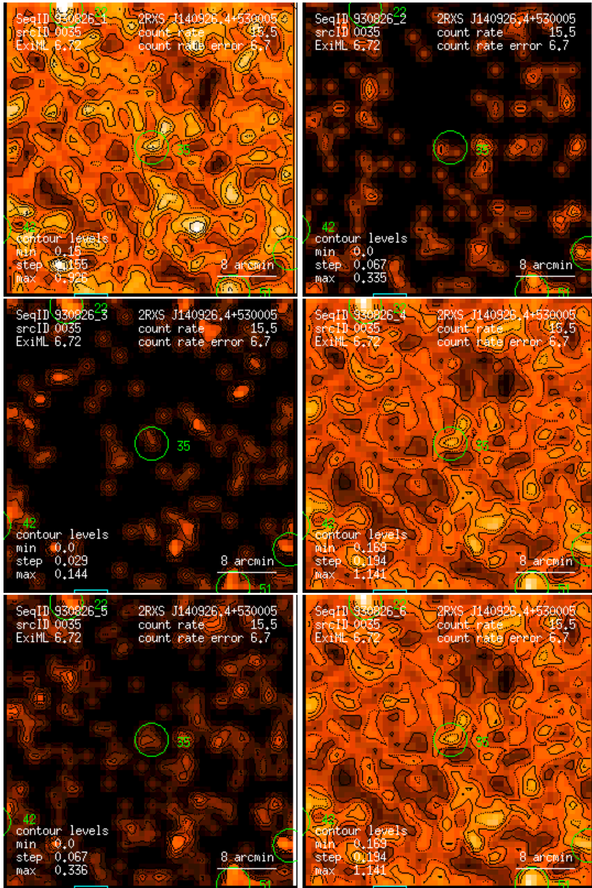
Figure 35: RASS 930826: detection 0035: band rate images, Gaussian filter: (1) PSPC channels 11 – 41, (2) 52 – 90, (3) 91 – 201, (4) 11 – 235, (5) 52 – 201, (6) 11 – 201. Broad band rates in counts/ks. Band rate contour levels in counts/ks/arcmin 2 .
