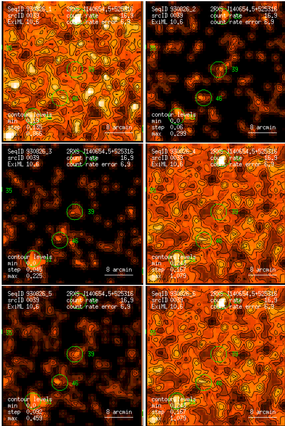
Figure 39: RASS 930826: detection 0039: band rate images, Gaussian filter: (1) PSPC channels 11 – 41, (2) 52 – 90, (3) 91 – 201, (4) 11 – 235, (5) 52 – 201, (6) 11 – 201. Broad band rates in counts/ks. Band rate contour levels in counts/ks/arcmin 2 .
