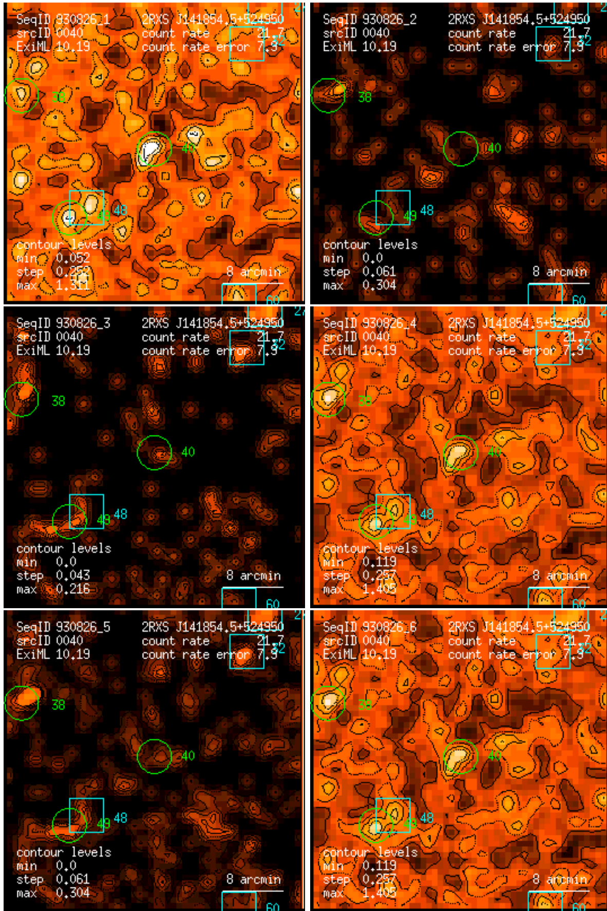
Figure 40: RASS 930826: detection 0040: band rate images, Gaussian filter: (1) PSPC channels 11 – 41, (2) 52 – 90, (3) 91 – 201, (4) 11 – 235, (5) 52 – 201, (6) 11 – 201. Broad band rates in counts/ks. Band rate contour levels in counts/ks/arcmin 2 .
