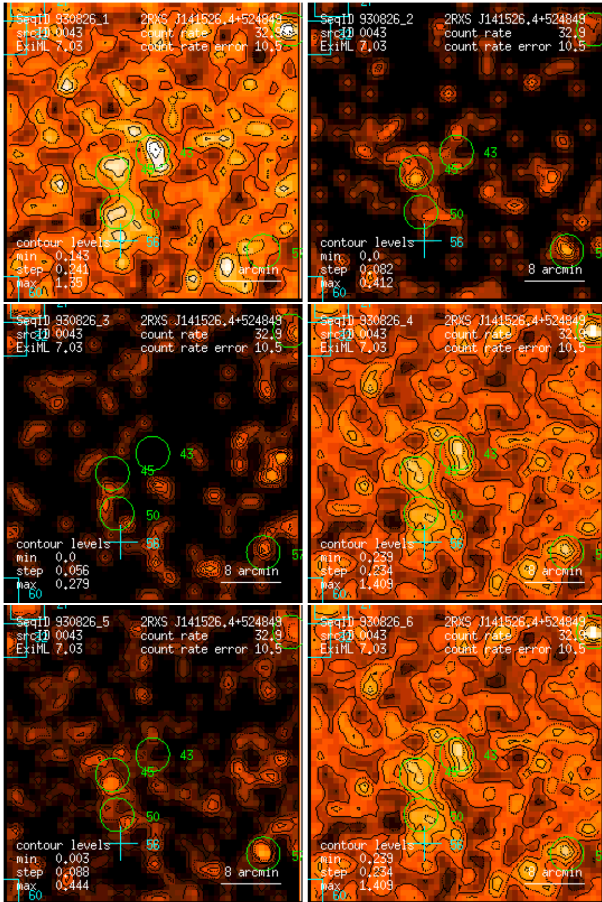
Figure 43: RASS 930826: detection 0043: band rate images, Gaussian filter: (1) PSPC channels 11 – 41, (2) 52 – 90, (3) 91 – 201, (4) 11 – 235, (5) 52 – 201, (6) 11 – 201. Broad band rates in counts/ks. Band rate contour levels in counts/ks/arcmin 2 .
