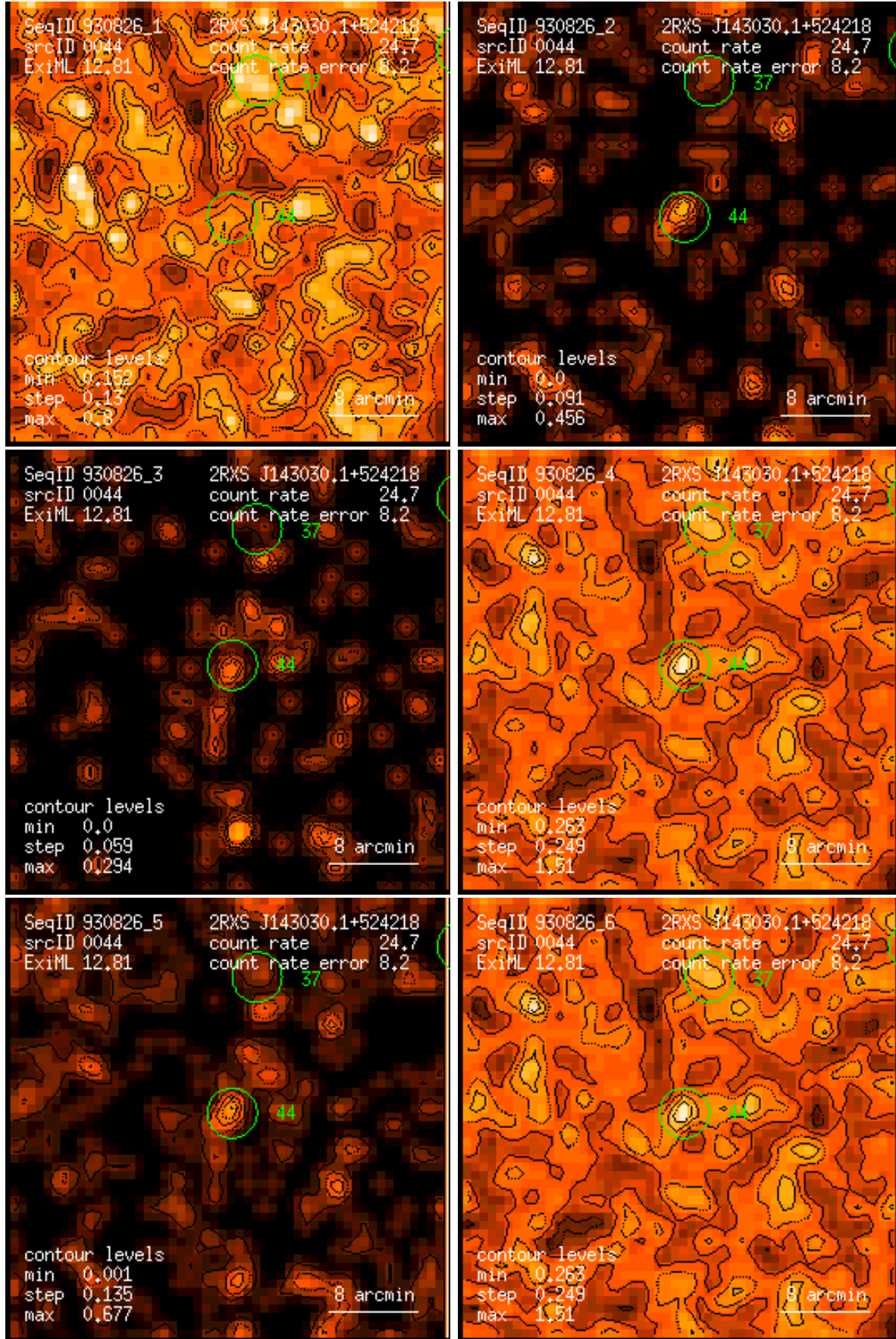
Figure 44: RASS 930826: detection 0044: band rate images, Gaussian filter: (1) PSPC channels 11 – 41, (2) 52 – 90, (3) 91 – 201, (4) 11 – 235, (5) 52 – 201, (6) 11 – 201. Broad band rates in counts/ks. Band rate contour levels in counts/ks/arcmin 2 .
