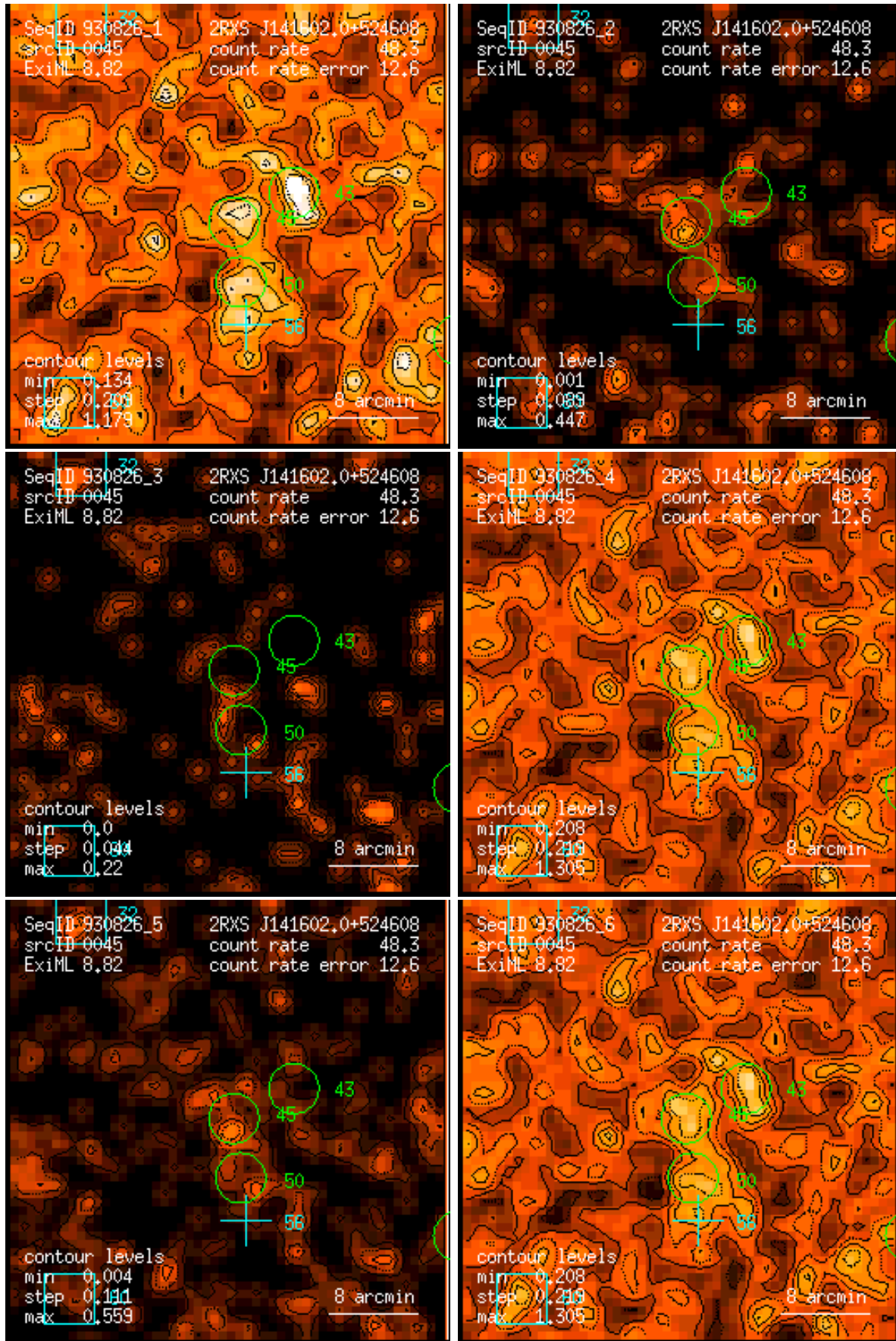
Figure 45: RASS 930826: detection 0045: band rate images, Gaussian filter: (1) PSPC channels 11 – 41, (2) 52 – 90, (3) 91 – 201, (4) 11 – 235, (5) 52 – 201, (6) 11 – 201. Broad band rates in counts/ks. Band rate contour levels in counts/ks/arcmin 2 .
