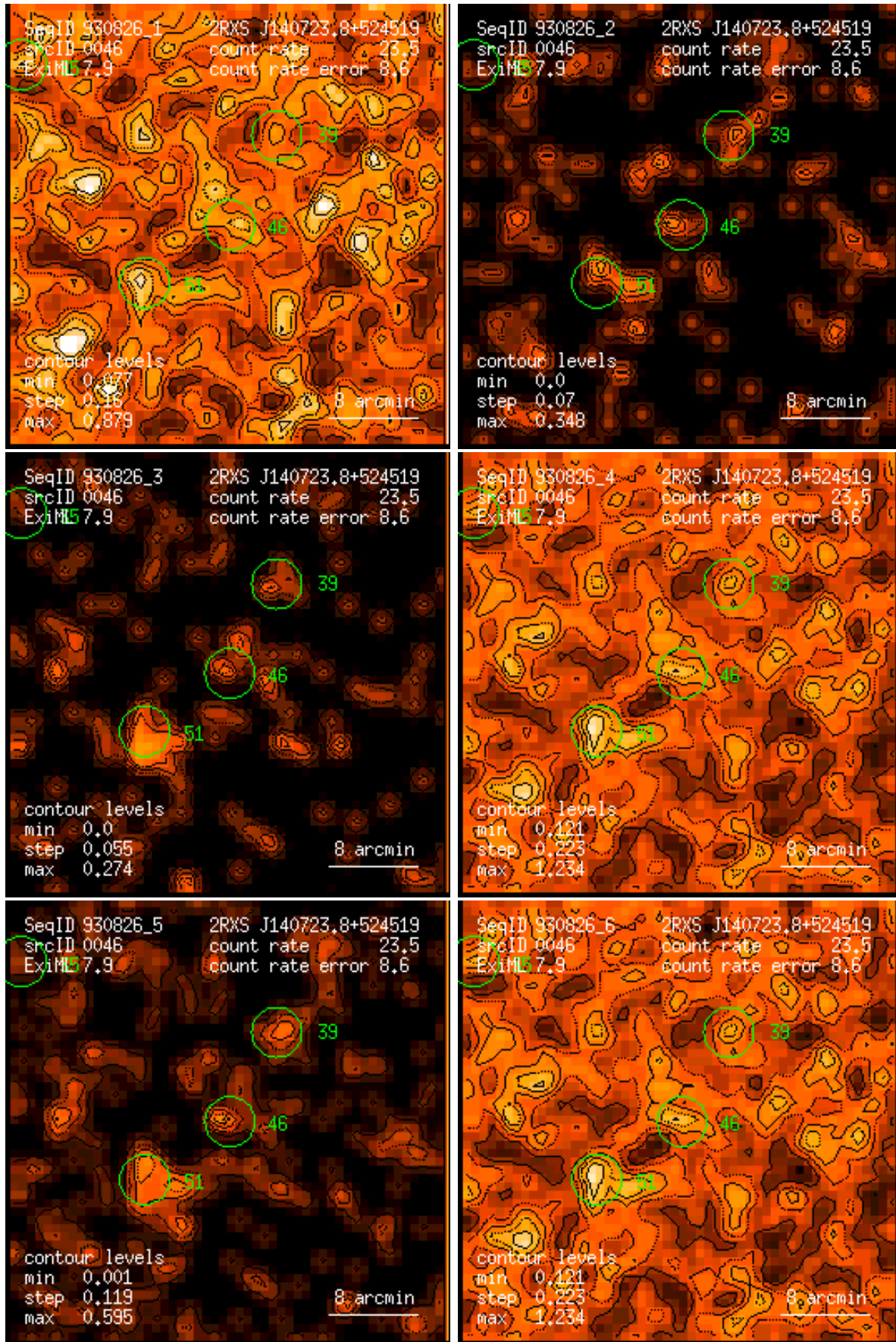
Figure 46: RASS 930826: detection 0046: band rate images, Gaussian filter: (1) PSPC channels 11 – 41, (2) 52 – 90, (3) 91 – 201, (4) 11 – 235, (5) 52 – 201, (6) 11 – 201. Broad band rates in counts/ks. Band rate contour levels in counts/ks/arcmin 2 .
