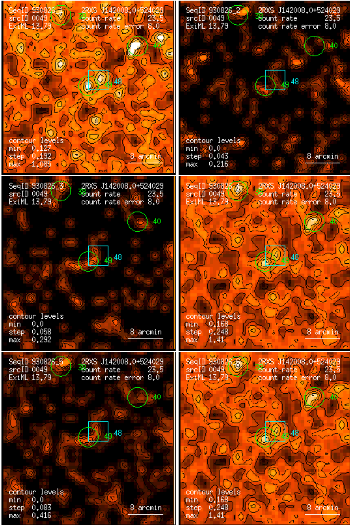
Figure 49: RASS 930826: detection 0049: band rate images, Gaussian filter: (1) PSPC channels 11 – 41, (2) 52 – 90, (3) 91 – 201, (4) 11 – 235, (5) 52 – 201, (6) 11 – 201. Broad band rates in counts/ks. Band rate contour levels in counts/ks/arcmin 2 .
