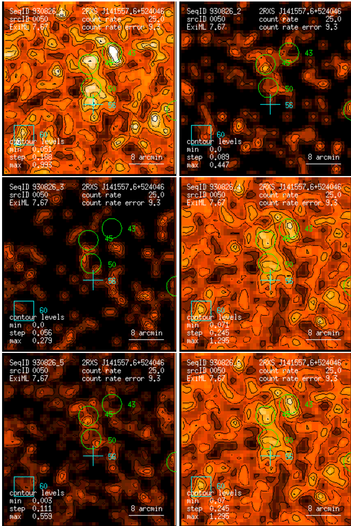
Figure 50: RASS 930826: detection 0050: band rate images, Gaussian filter: (1) PSPC channels 11 – 41, (2) 52 – 90, (3) 91 – 201, (4) 11 – 235, (5) 52 – 201, (6) 11 – 201. Broad band rates in counts/ks. Band rate contour levels in counts/ks/arcmin 2 .
