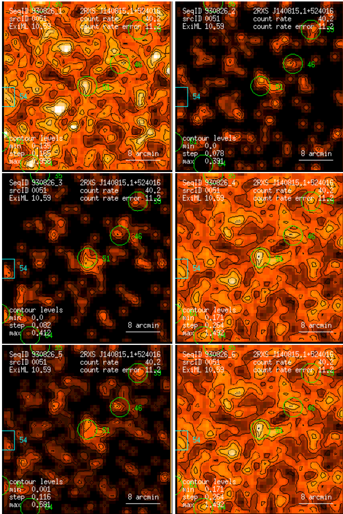
Figure 51: RASS 930826: detection 0051: band rate images, Gaussian filter: (1) PSPC channels 11 – 41, (2) 52 – 90, (3) 91 – 201, (4) 11 – 235, (5) 52 – 201, (6) 11 – 201. Broad band rates in counts/ks. Band rate contour levels in counts/ks/arcmin 2 .
