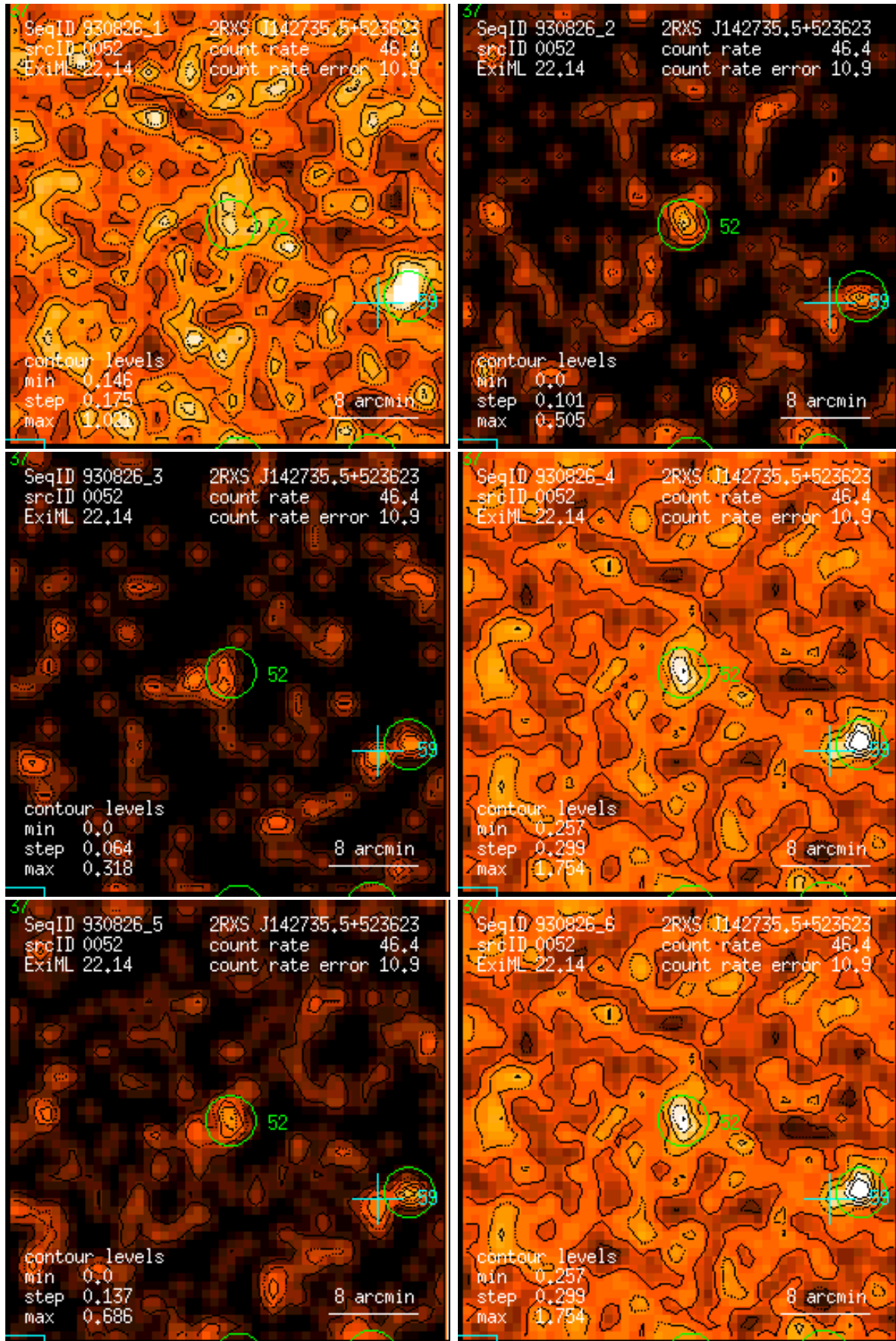
Figure 52: RASS 930826: detection 0052: band rate images, Gaussian filter: (1) PSPC channels 11 – 41, (2) 52 – 90, (3) 91 – 201, (4) 11 – 235, (5) 52 – 201, (6) 11 – 201. Broad band rates in counts/ks. Band rate contour levels in counts/ks/arcmin 2 .
