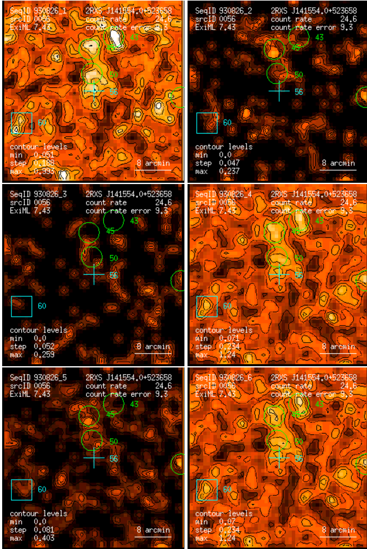
Figure 56: RASS 930826: detection 0056: band rate images, Gaussian filter: (1) PSPC channels 11 – 41, (2) 52 – 90, (3) 91 – 201, (4) 11 – 235, (5) 52 – 201, (6) 11 – 201. Broad band rates in counts/ks. Band rate contour levels in counts/ks/arcmin 2 .
