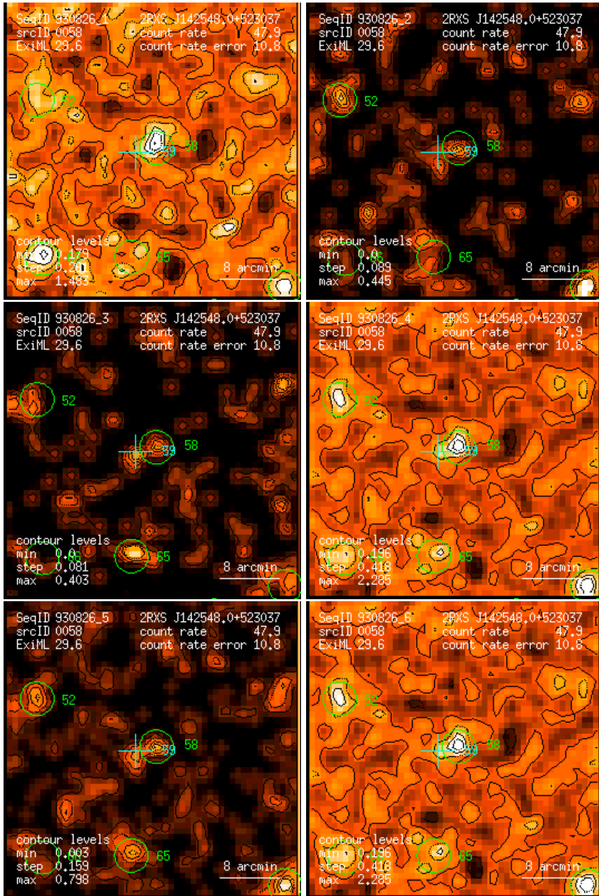
Figure 58: RASS 930826: detection 0058: band rate images, Gaussian filter: (1) PSPC channels 11 – 41, (2) 52 – 90, (3) 91 – 201, (4) 11 – 235, (5) 52 – 201, (6) 11 – 201. Broad band rates in counts/ks. Band rate contour levels in counts/ks/arcmin 2 .
