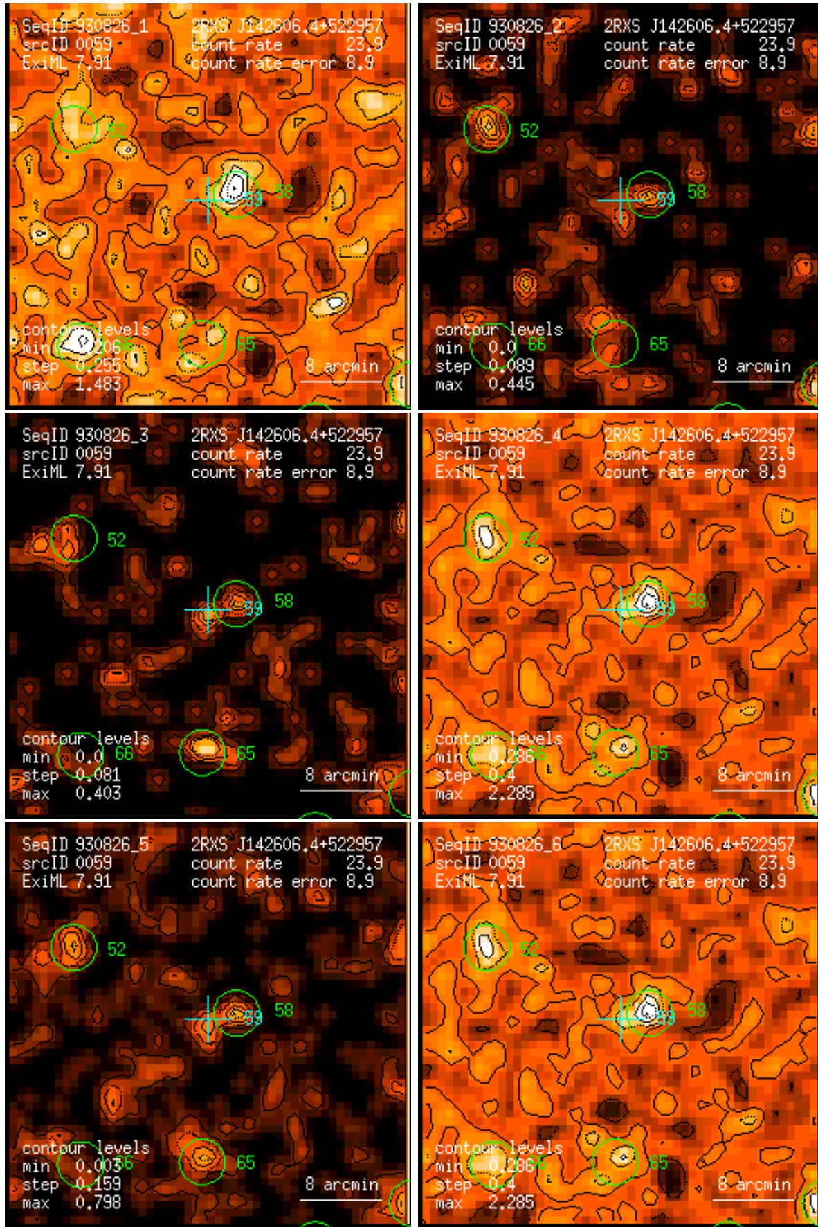
Figure 59: RASS 930826: detection 0059: band rate images, Gaussian filter: (1) PSPC channels 11 – 41, (2) 52 – 90, (3) 91 – 201, (4) 11 – 235, (5) 52 – 201, (6) 11 – 201. Broad band rates in counts/ks. Band rate contour levels in counts/ks/arcmin 2 .
