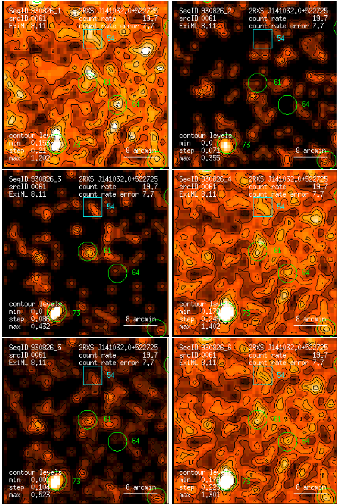
Figure 61: RASS 930826: detection 0061: band rate images, Gaussian filter: (1) PSPC channels 11 – 41, (2) 52 – 90, (3) 91 – 201, (4) 11 – 235, (5) 52 – 201, (6) 11 – 201. Broad band rates in counts/ks. Band rate contour levels in counts/ks/arcmin 2 .
