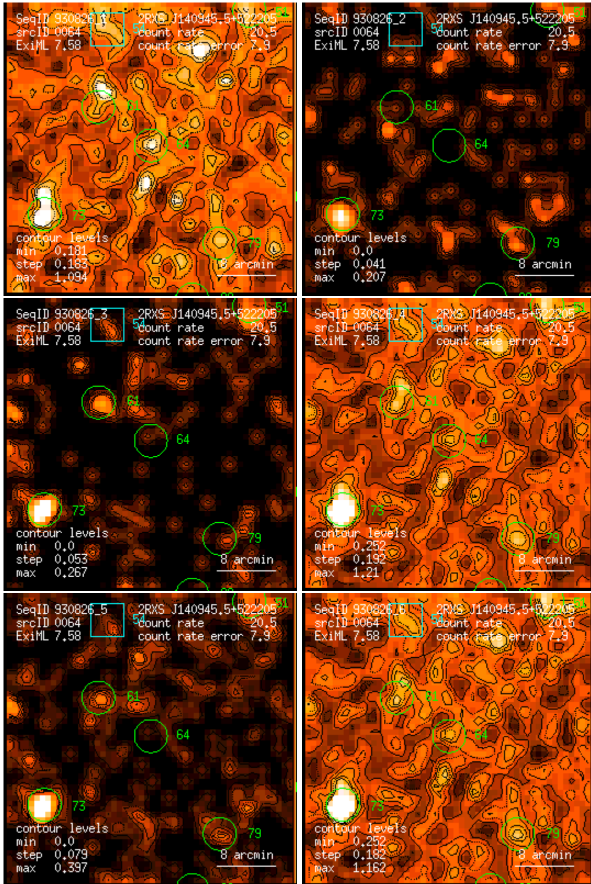
Figure 64: RASS 930826: detection 0064: band rate images, Gaussian filter: (1) PSPC channels 11 – 41, (2) 52 – 90, (3) 91 – 201, (4) 11 – 235, (5) 52 – 201, (6) 11 – 201. Broad band rates in counts/ks. Band rate contour levels in counts/ks/arcmin 2 .
