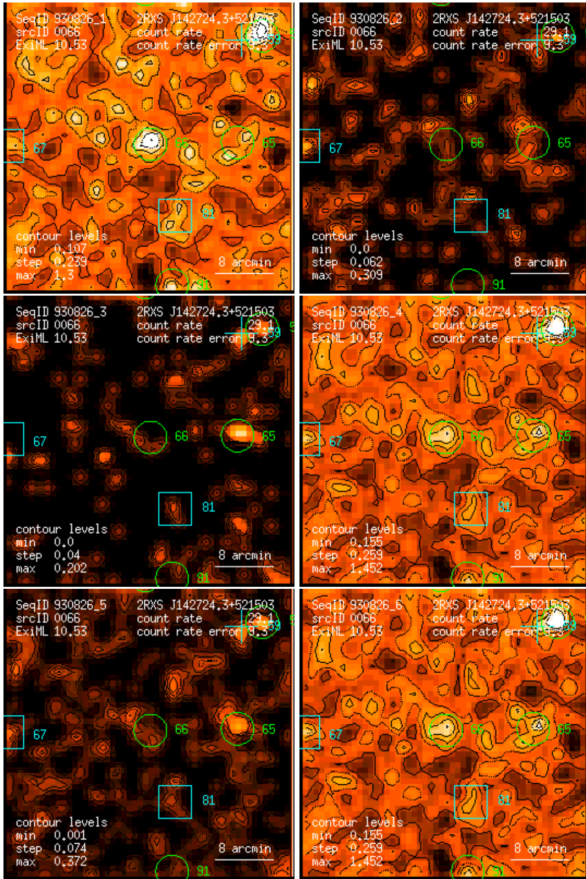
Figure 66: RASS 930826: detection 0066: band rate images, Gaussian filter: (1) PSPC channels 11 – 41, (2) 52 – 90, (3) 91 – 201, (4) 11 – 235, (5) 52 – 201, (6) 11 – 201. Broad band rates in counts/ks. Band rate contour levels in counts/ks/arcmin 2 .
