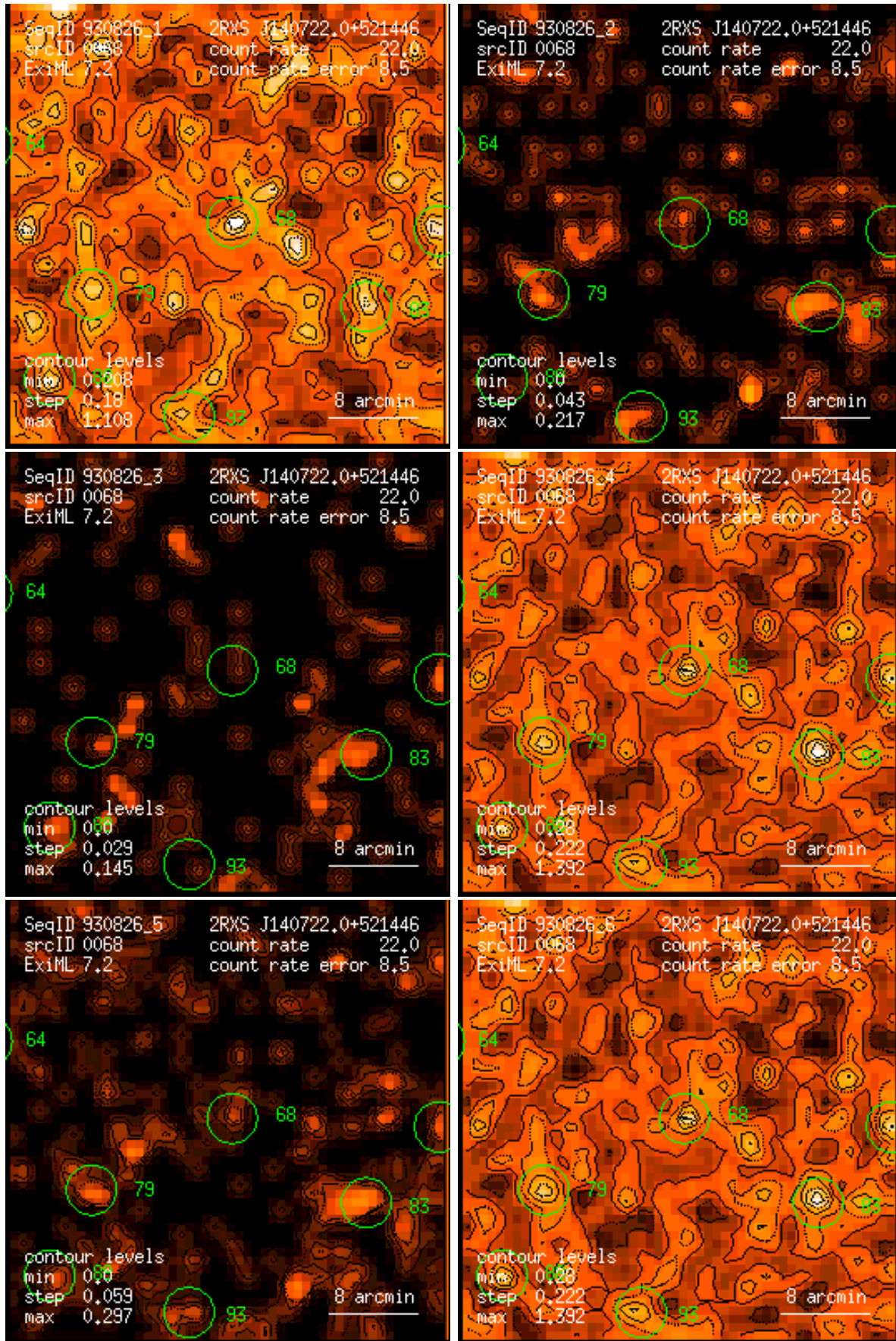
Figure 68: RASS 930826: detection 0068: band rate images, Gaussian filter: (1) PSPC channels 11 – 41, (2) 52 – 90, (3) 91 – 201, (4) 11 – 235, (5) 52 – 201, (6) 11 – 201. Broad band rates in counts/ks. Band rate contour levels in counts/ks/arcmin 2 .
