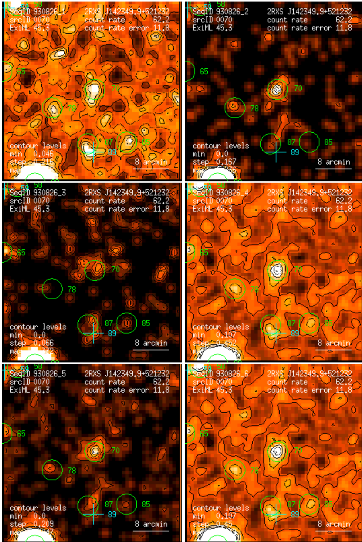
Figure 70: RASS 930826: detection 0070: band rate images, Gaussian filter: (1) PSPC channels 11 – 41, (2) 52 – 90, (3) 91 – 201, (4) 11 – 235, (5) 52 – 201, (6) 11 – 201. Broad band rates in counts/ks. Band rate contour levels in counts/ks/arcmin 2 .
