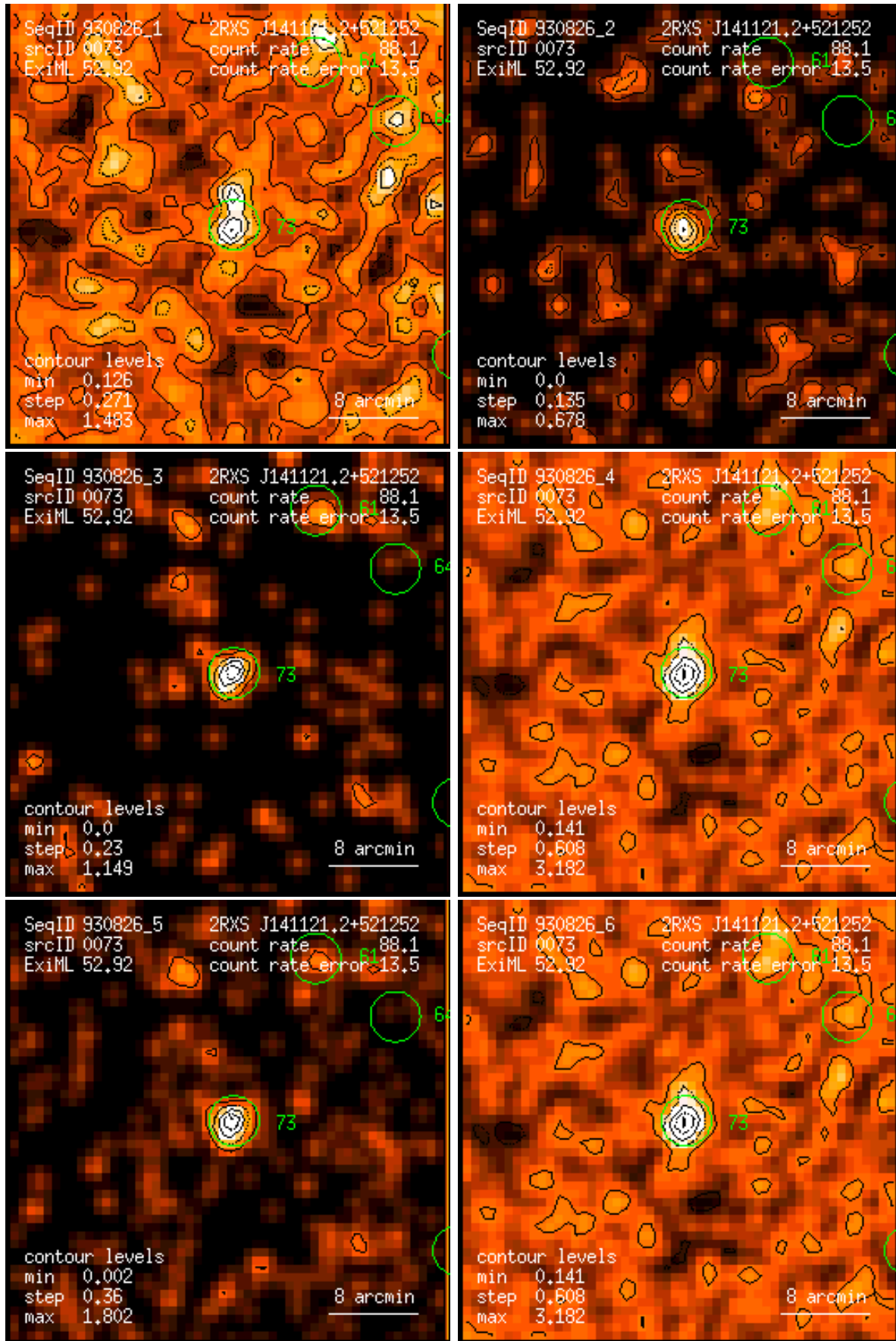
Figure 73: RASS 930826: detection 0073: band rate images, Gaussian filter: (1) PSPC channels 11 – 41, (2) 52 – 90, (3) 91 – 201, (4) 11 – 235, (5) 52 – 201, (6) 11 – 201. Broad band rates in counts/ks. Band rate contour levels in counts/ks/arcmin 2 .
