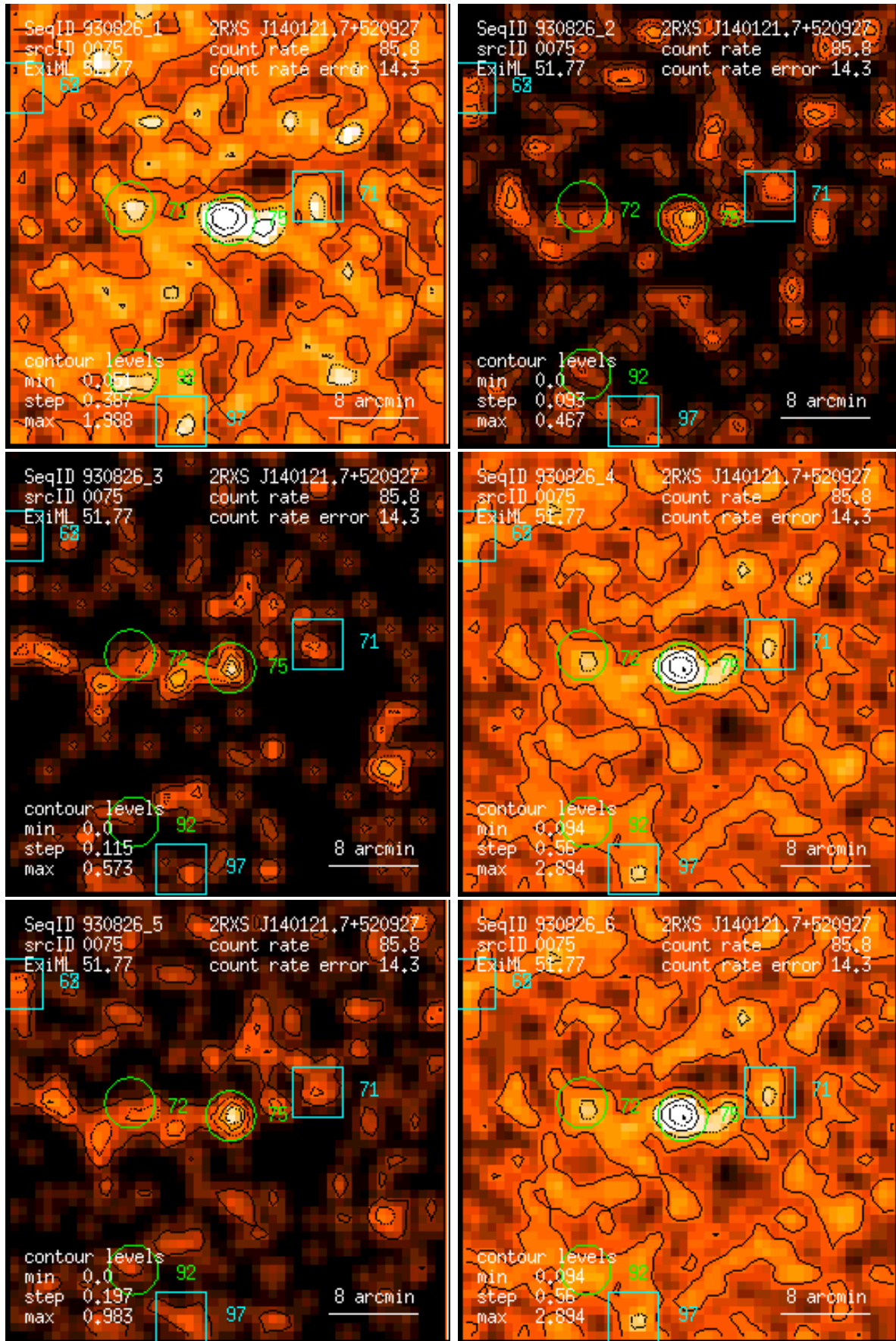
Figure 75: RASS 930826: detection 0075: band rate images, Gaussian filter: (1) PSPC channels 11 – 41, (2) 52 – 90, (3) 91 – 201, (4) 11 – 235, (5) 52 – 201, (6) 11 – 201. Broad band rates in counts/ks. Band rate contour levels in counts/ks/arcmin 2 .
